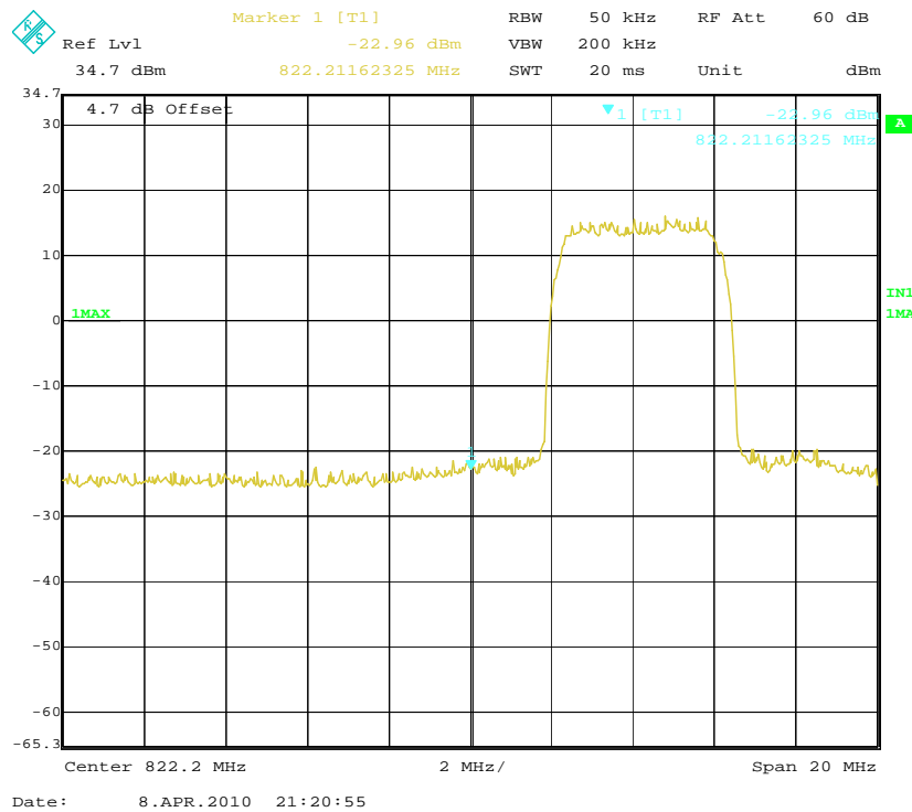
HSUPA channel 4132 left band edge
