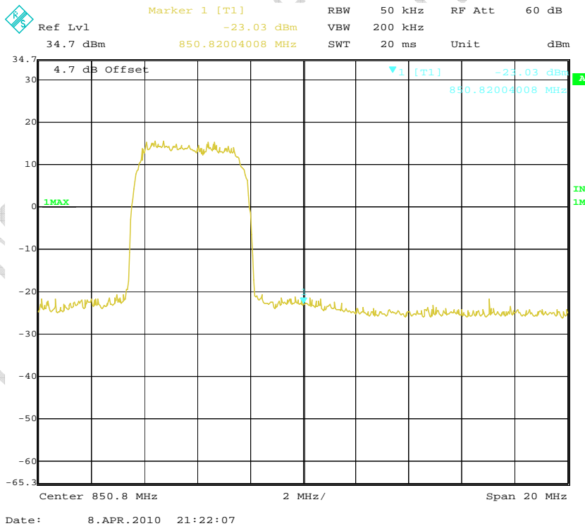
HSUPA channel 4233 right band edge
