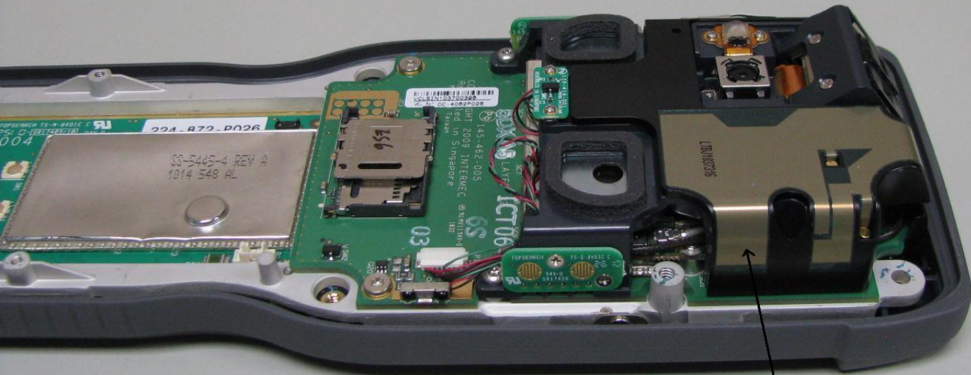
UMTS ANTENNA
