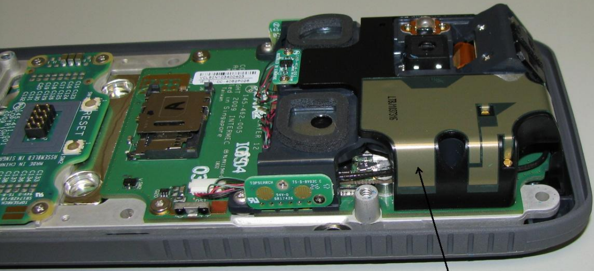
UMTS ANTENNA
