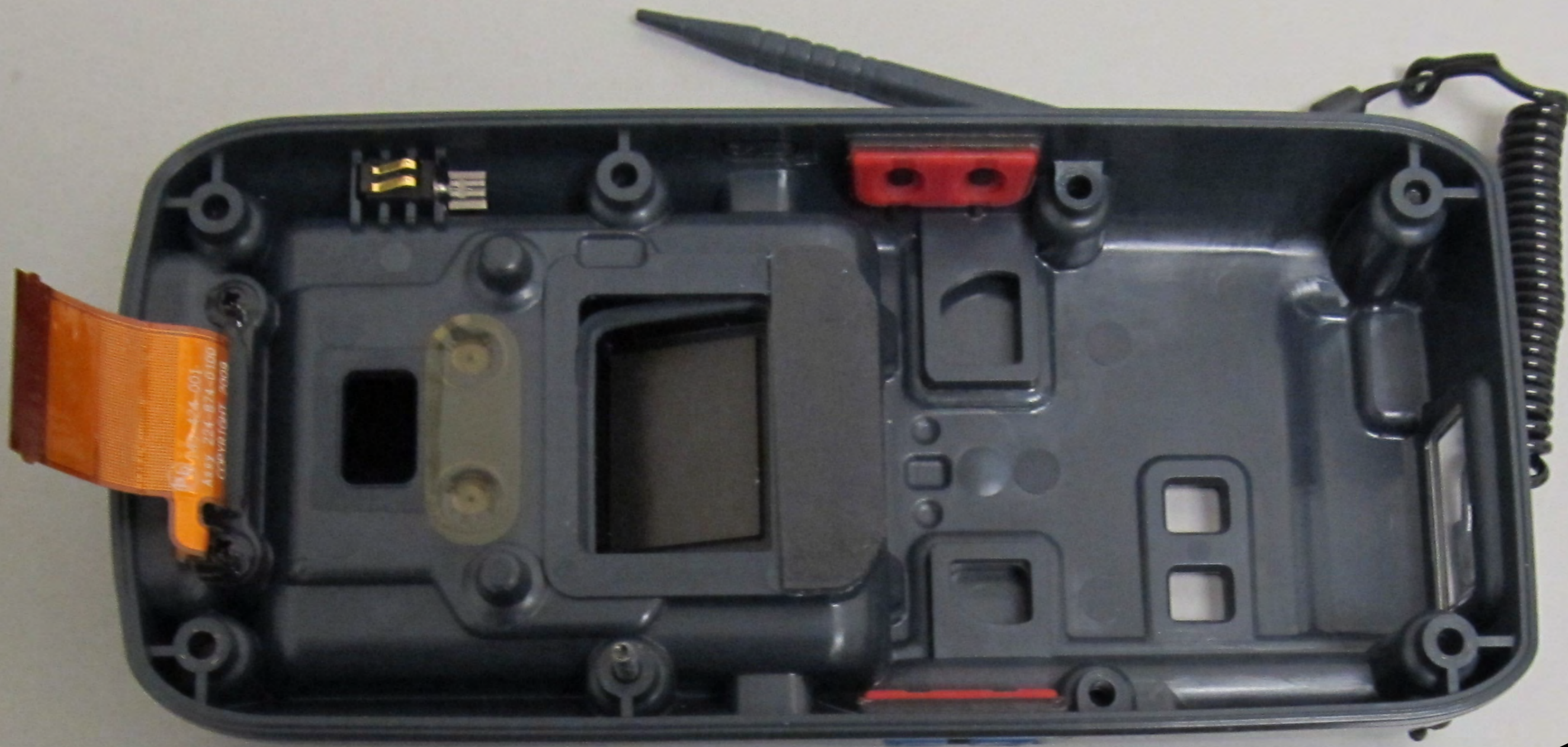
WLAN/Bluetooth Antenna
