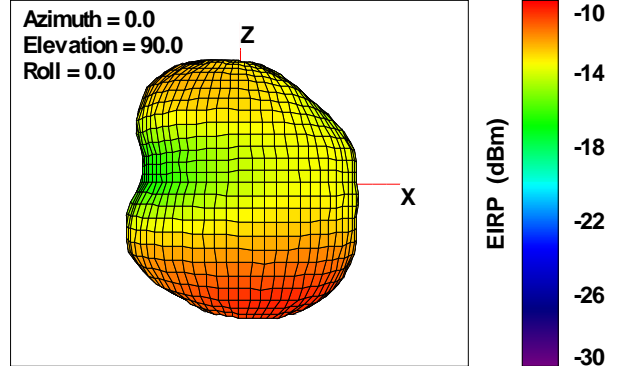
Total ERP, Left Side View
