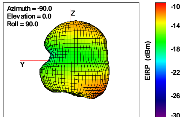
Total ERP, Back Face View
