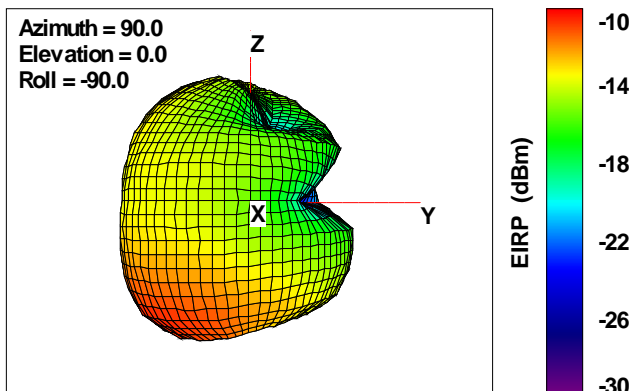
Total ERP, Front Face View
