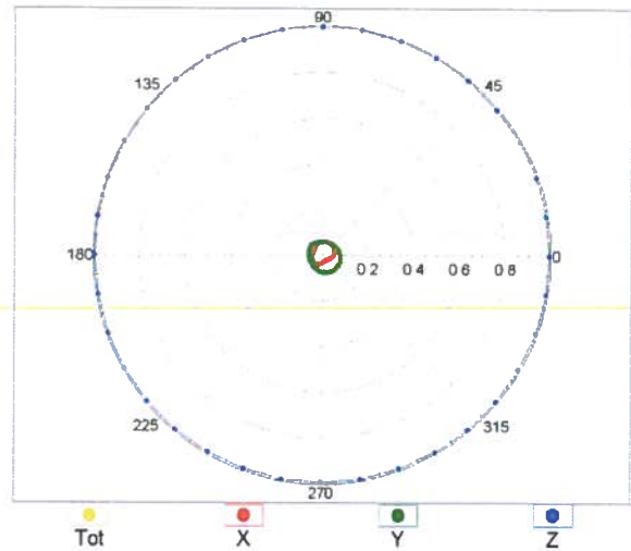
f=2500 MHz, R22, 90°
