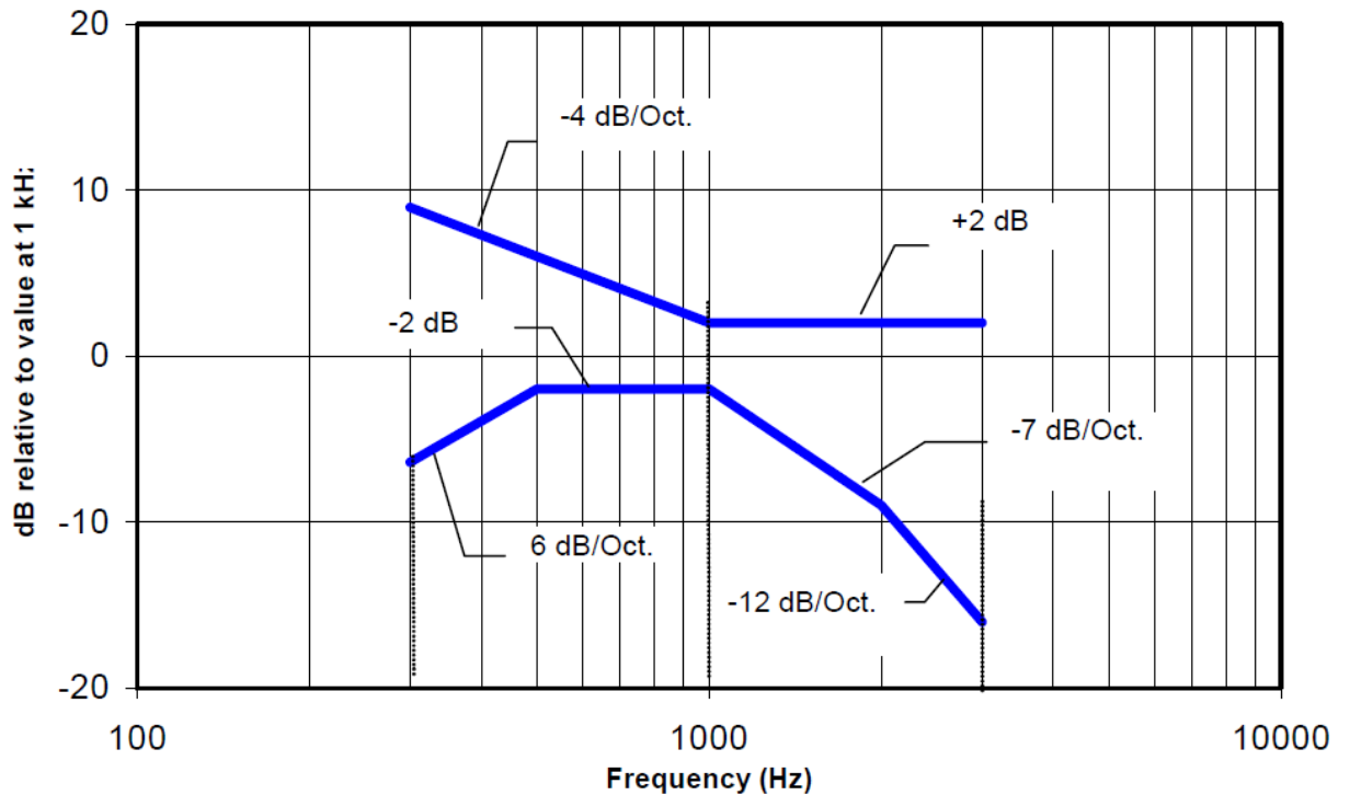
Figure 8.2—Magnetic field frequency response for WDs with a field that exceeds -15 \text{ dB(A/m)} at 1 kHz
