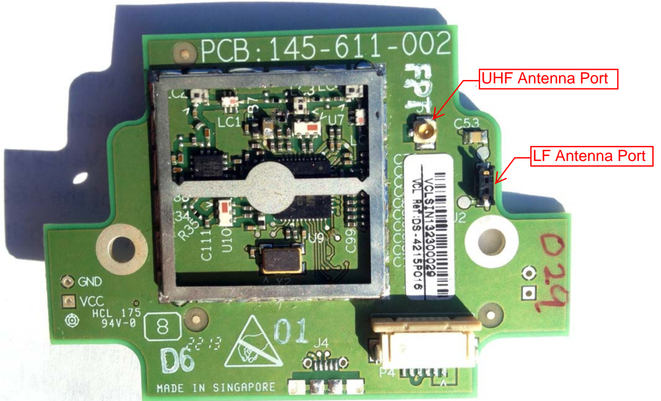
Main Board – Bottom Side, Shield Removed
