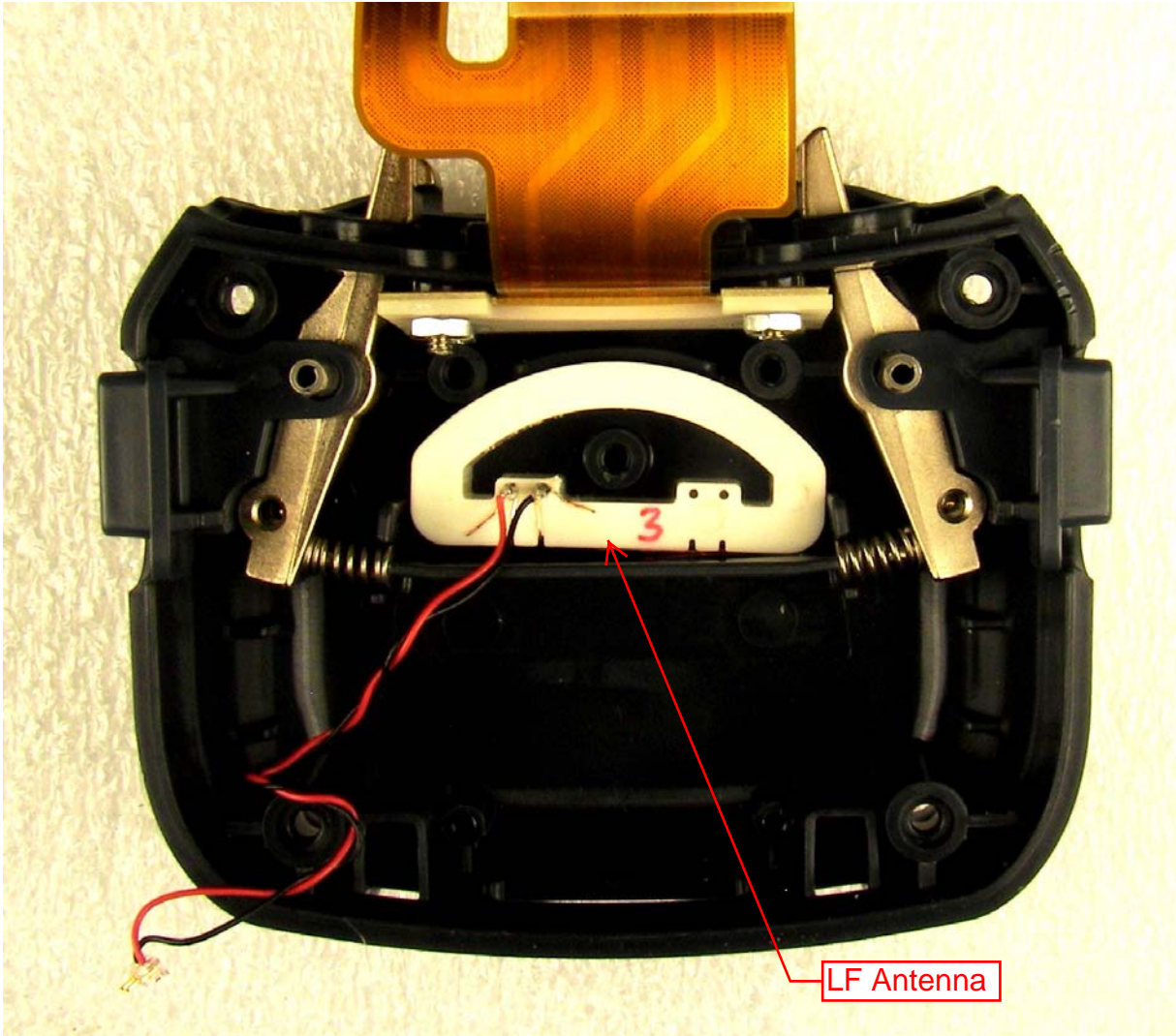
LF antenna, retaining plastic removed
