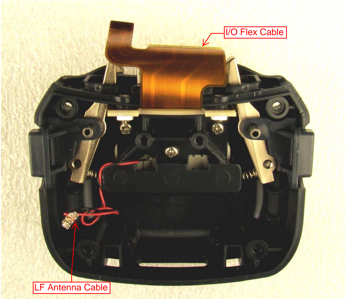
Mechanical layout showing LF antenna under retaining plastic
