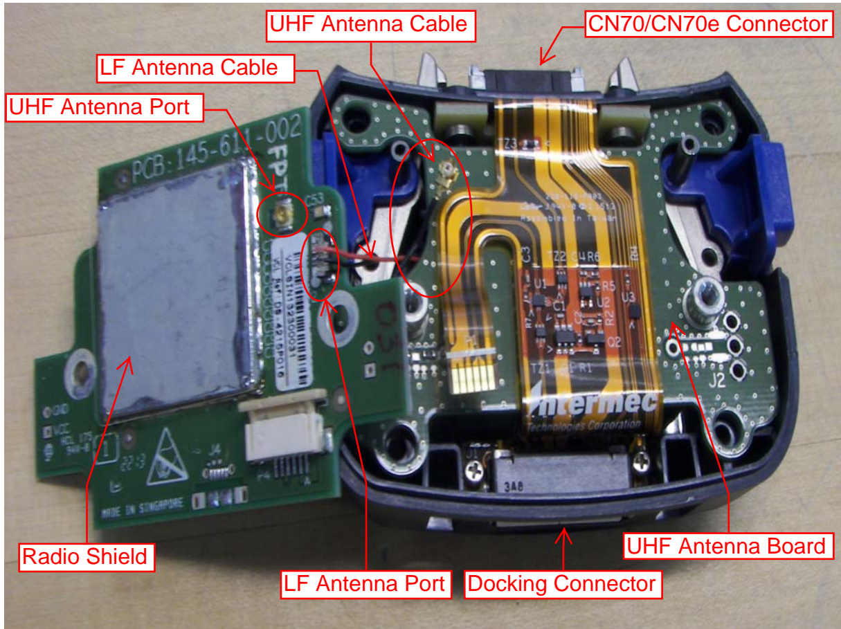
Main Board Removed
