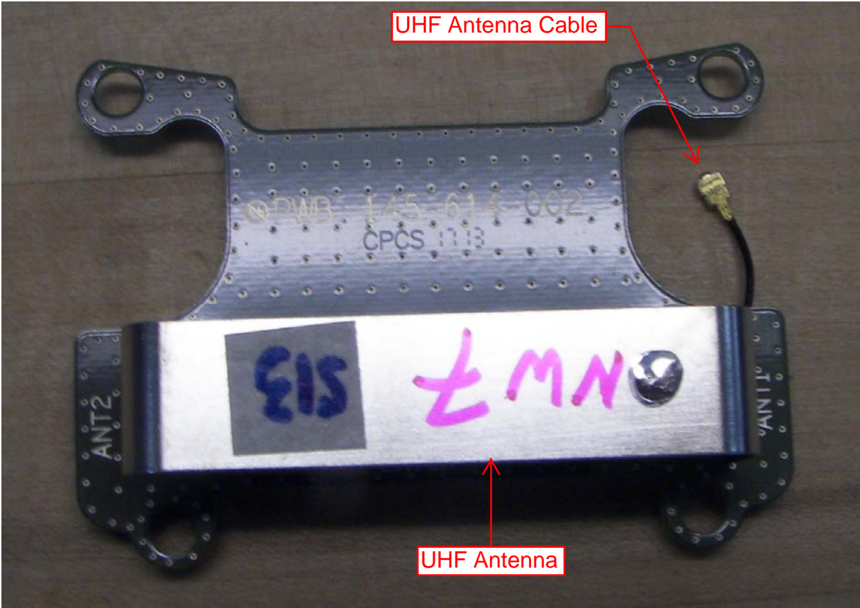
UHF Antenna Board – Bottom Side
