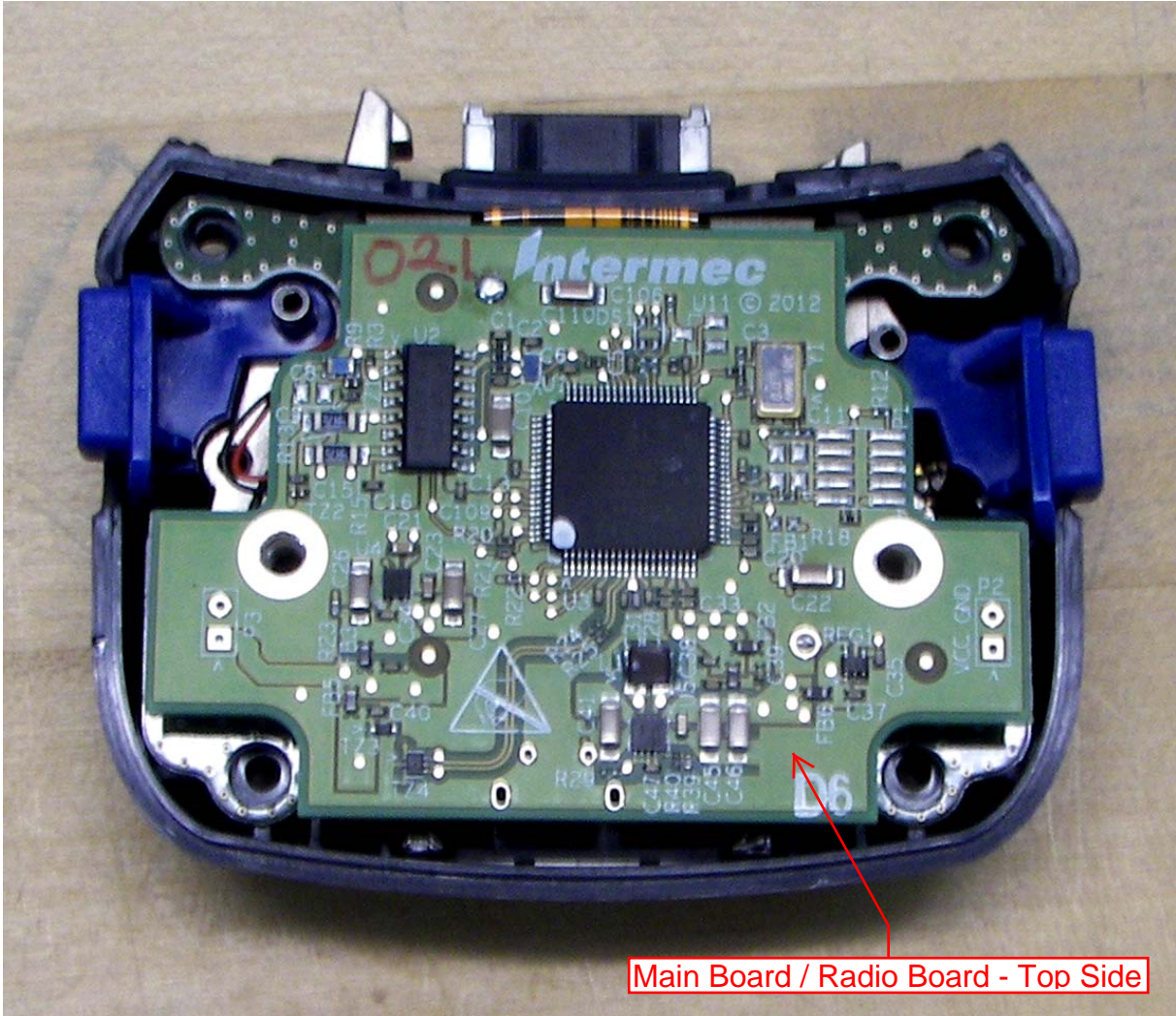
Top Enclosure Removed
