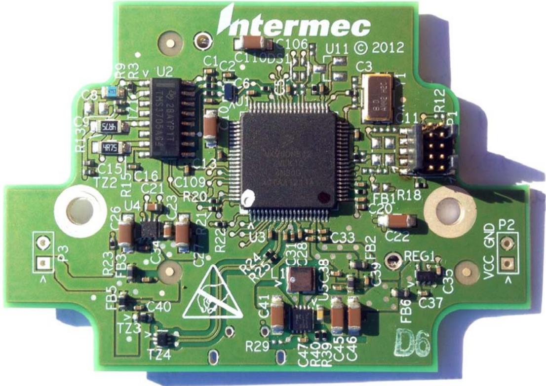
Main Board – Top Side
