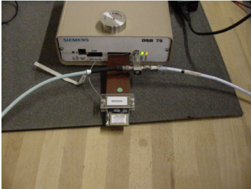
Picture 3 : Setup for conducted tests (setup 01s140a02)
