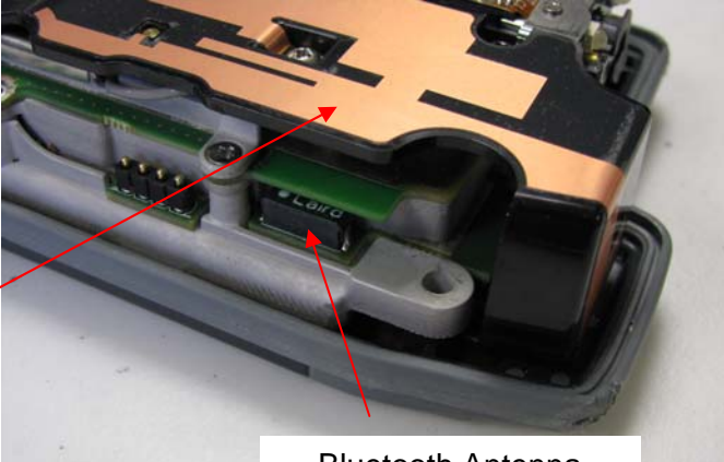
Bluetooth Antenna
