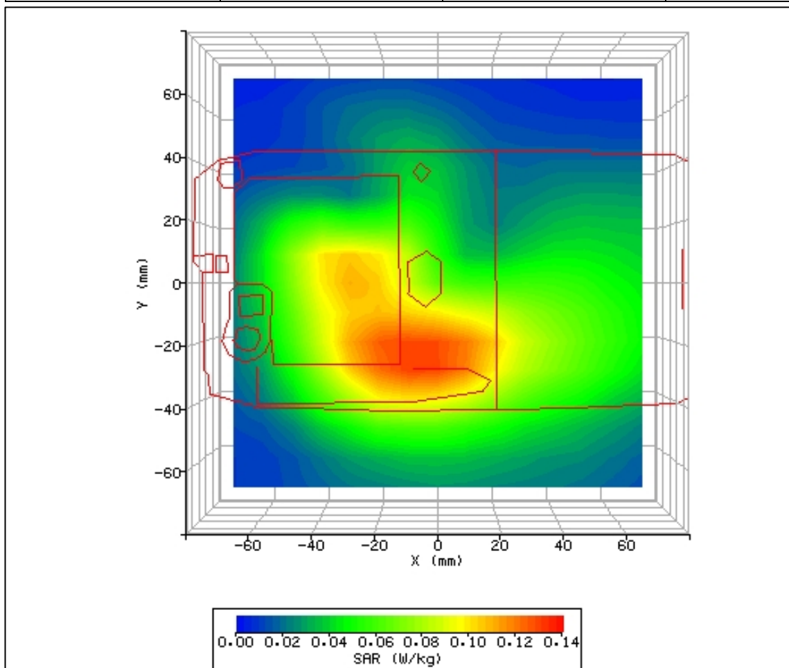
Figure 14: SAR Body GPRSTesting Results for the Intermec CN3 Mobile Computer in Rear Facing Phantom Position; Tested at 836.4MHz (850MHz GSM Middle Channel) with 15.0mm Separation.
