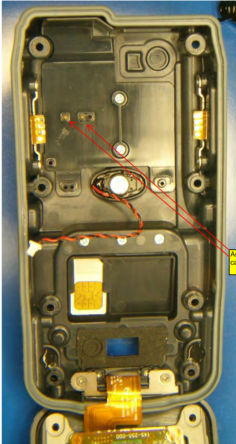
CN3 Case Back with MC75 Antenna Installed
