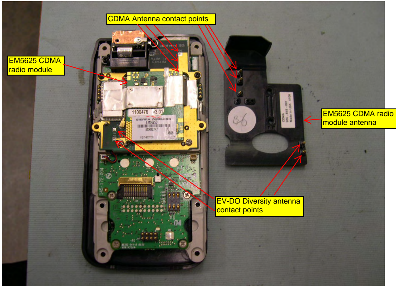
CN3 with EM5625 Antenna removed from back case
