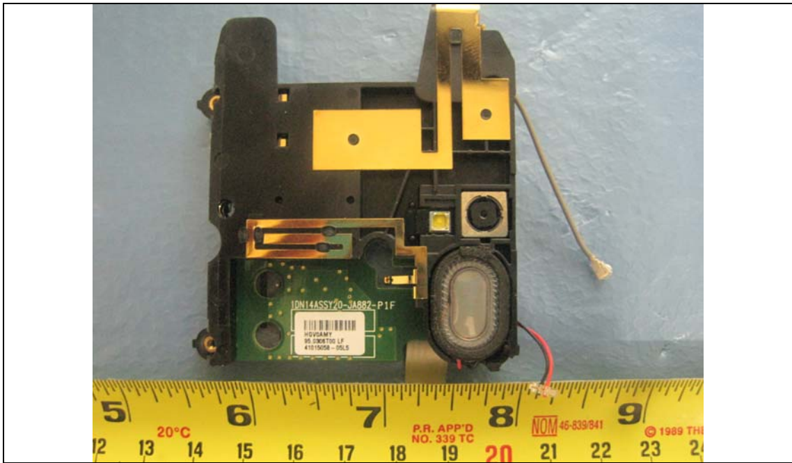
Antenna board Bottom View 1
