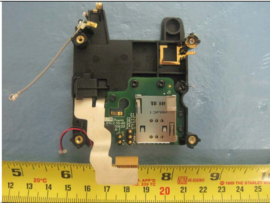
Antenna board Top View 1
