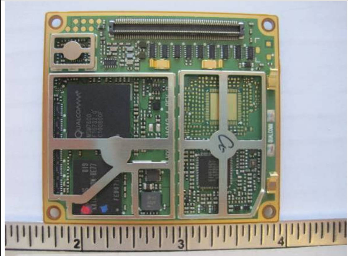
PCBA 2 Bottom View
