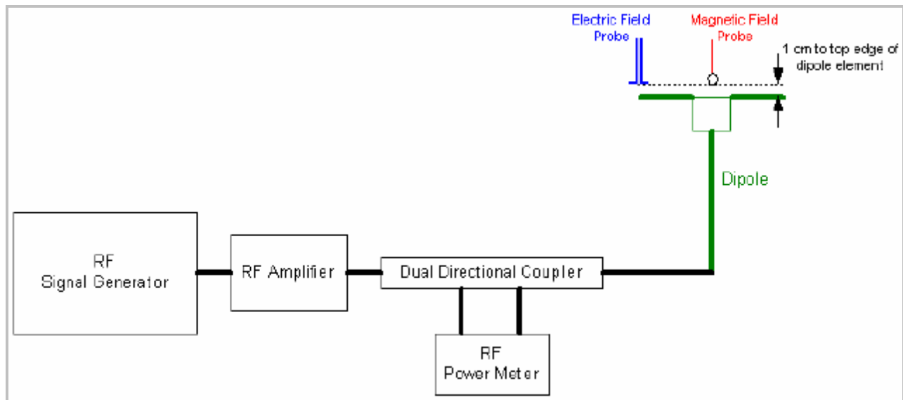
Setup diagram
