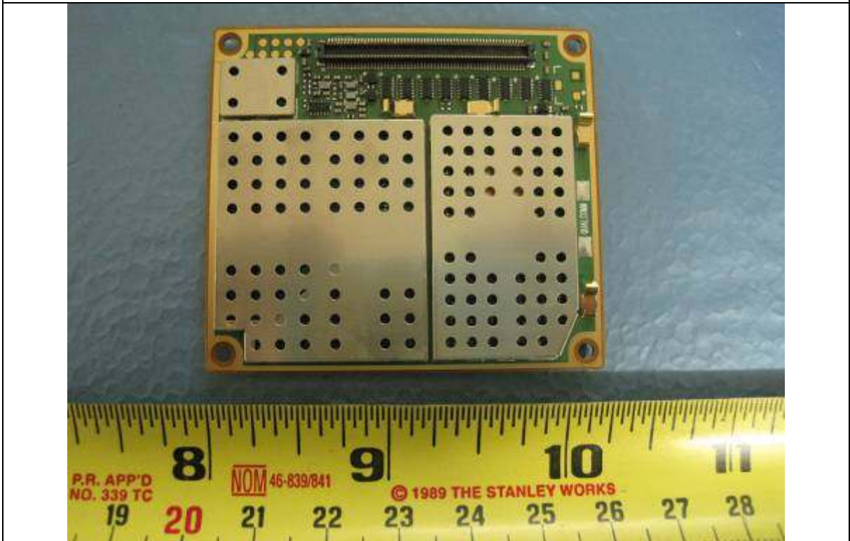
PCBA 2 Bottom View
