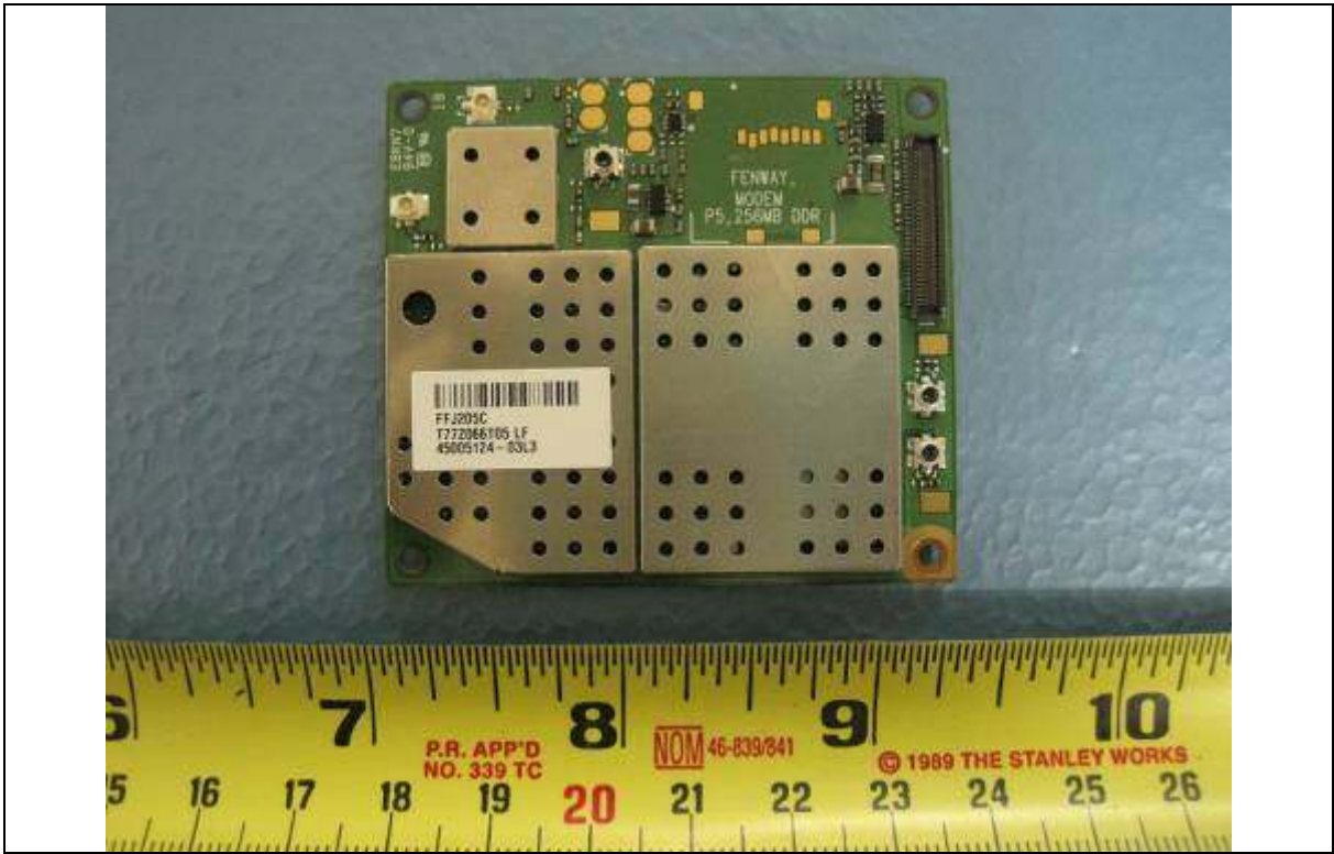
PCBA 2 Top View
