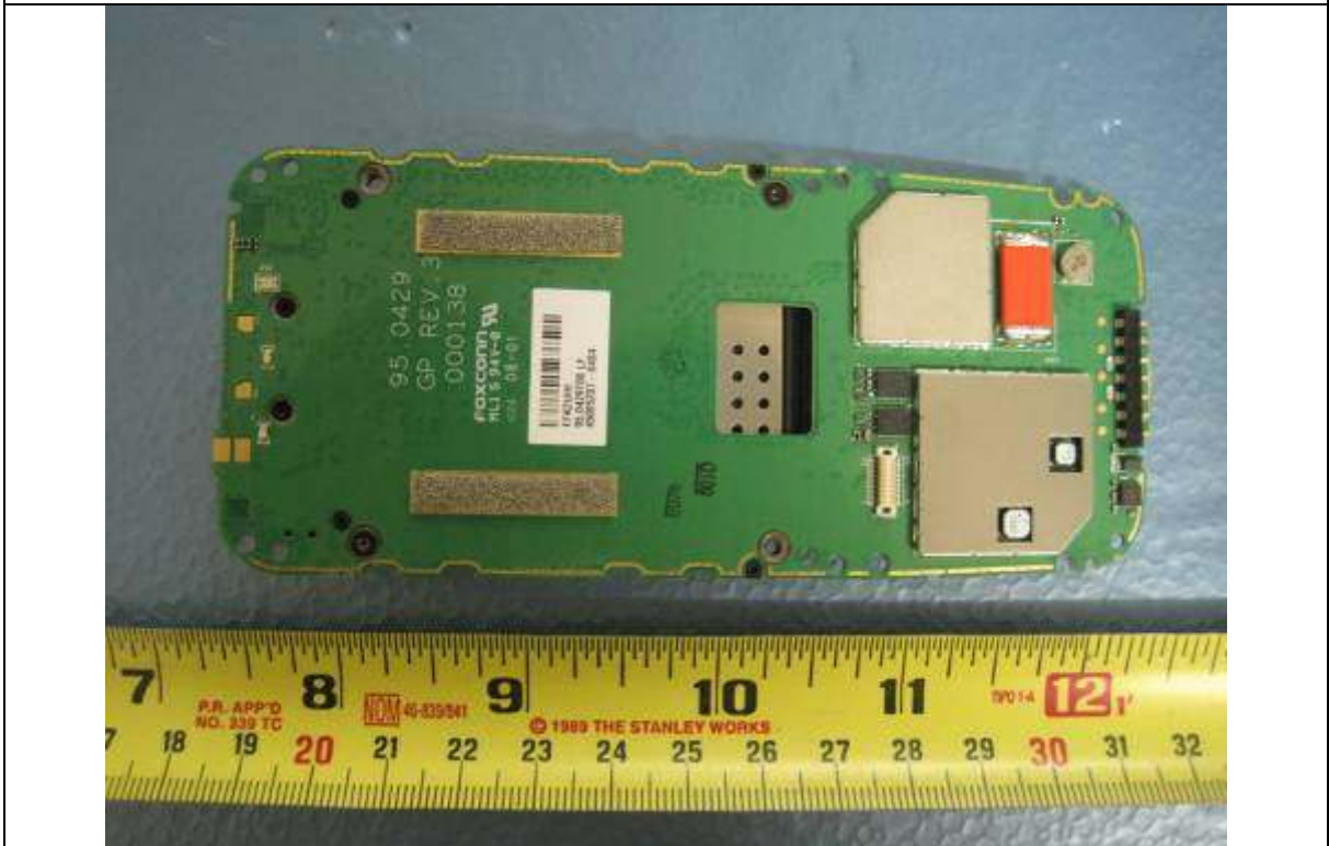
PCBA 1 Bottom View
