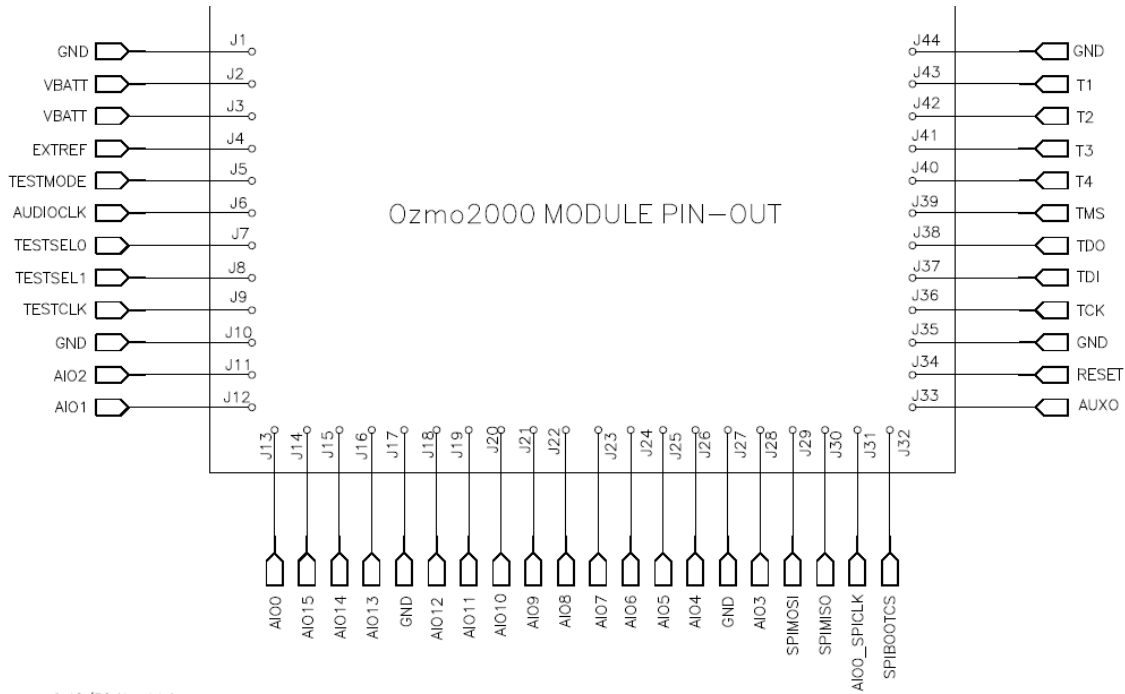
Figure 2 Module Pinout (Top View)
