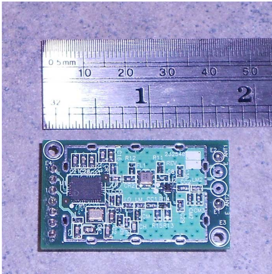
433.92 MHz TRANSCEIVER MODULE, PCB FRONT AND BACK.
