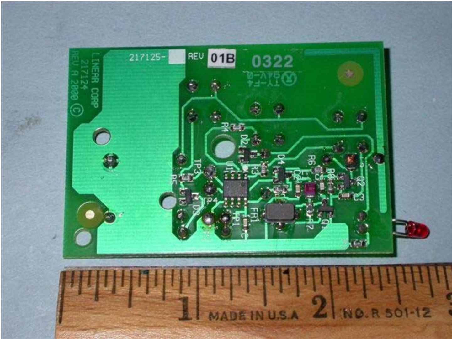
PCB Assembly, Back View, WT-30 Transmitter
