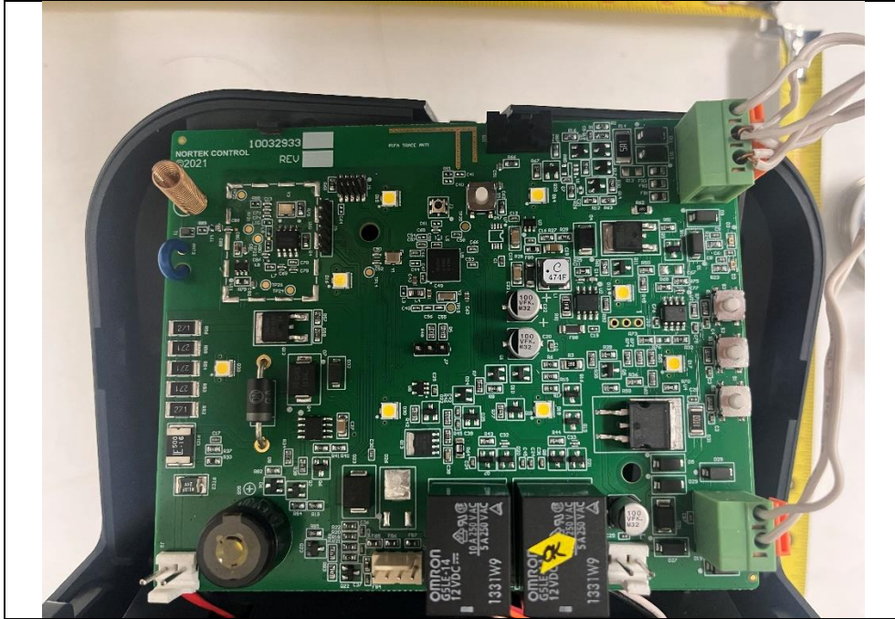
EUT cover view -1
