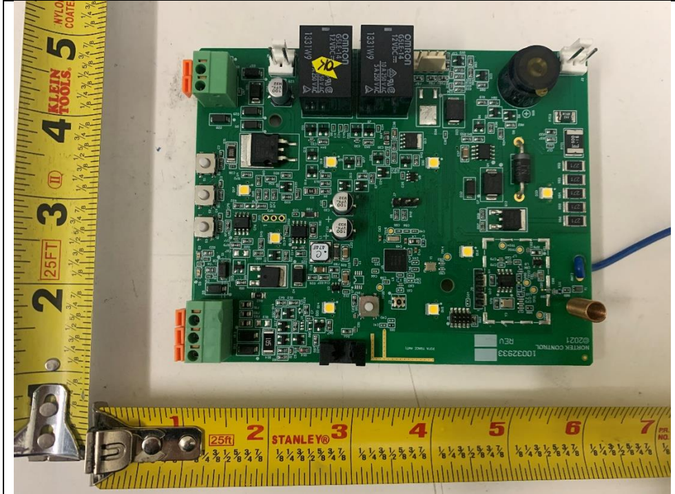
EUT Main PCBA Top View
