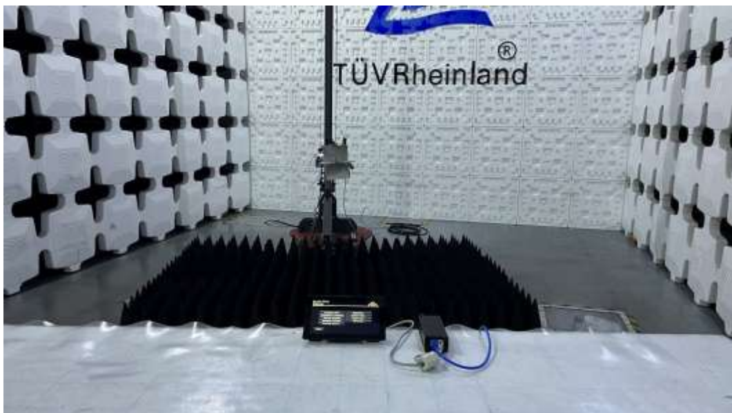
Photograph 4: Set-up photo for Radiated Emission, Above 1GHz
