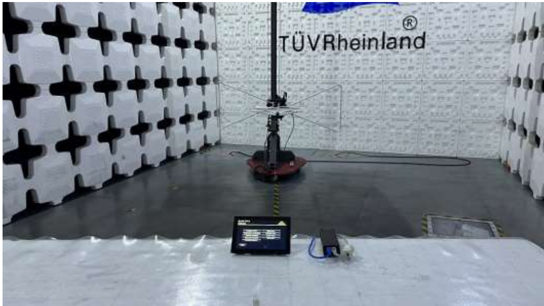
Photograph 3: Set-up photo for Radiated Emission, Below 1GHz
