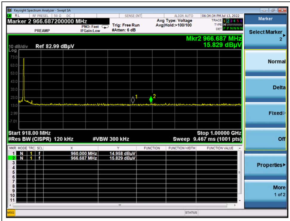
(920MHz, PEAK)
