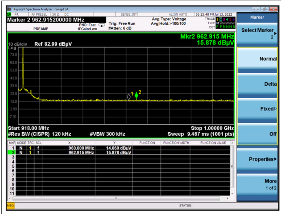
(912MHz, PEAK)
