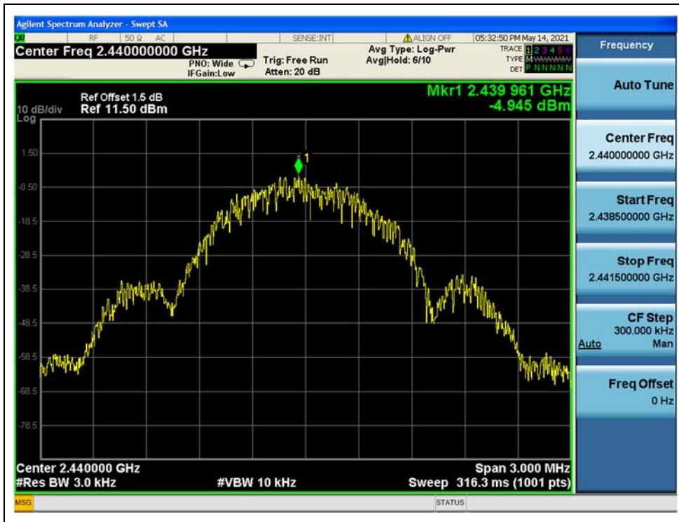
(Channel = 19, 2440MHz)
