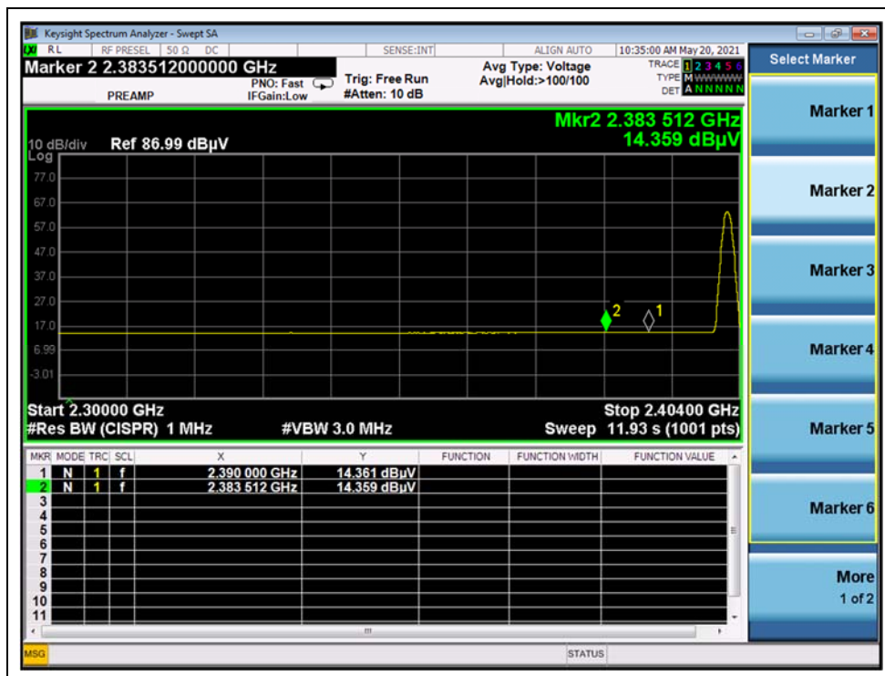
(AVG, Channel = 0)
