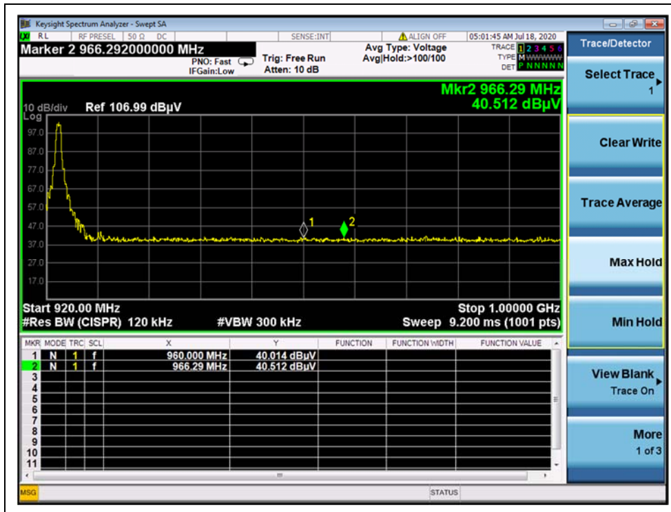
(922MHz, PEAK)
