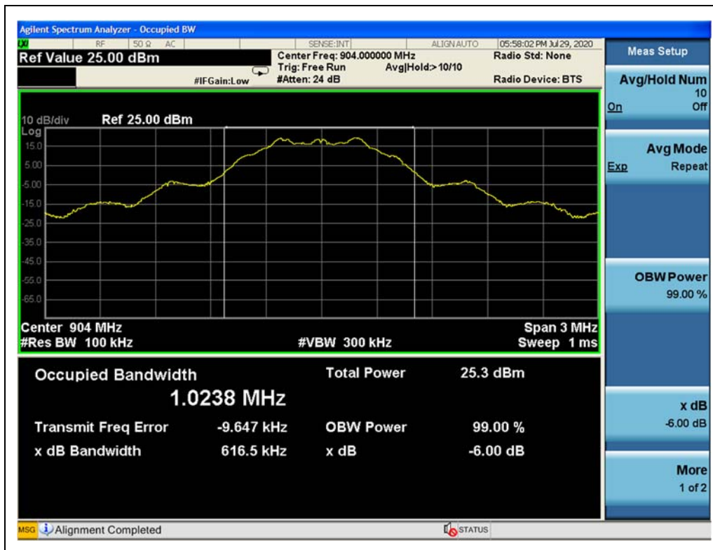
(904MHz)
