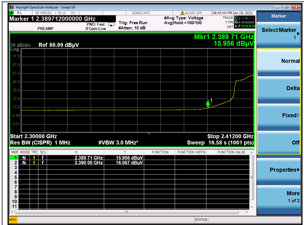
(AVG,Channel = 1, 802.11n(HT20))
