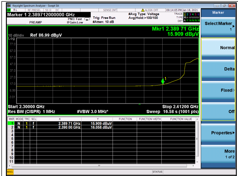
(AVG,Channel = 1, 802.11g)
