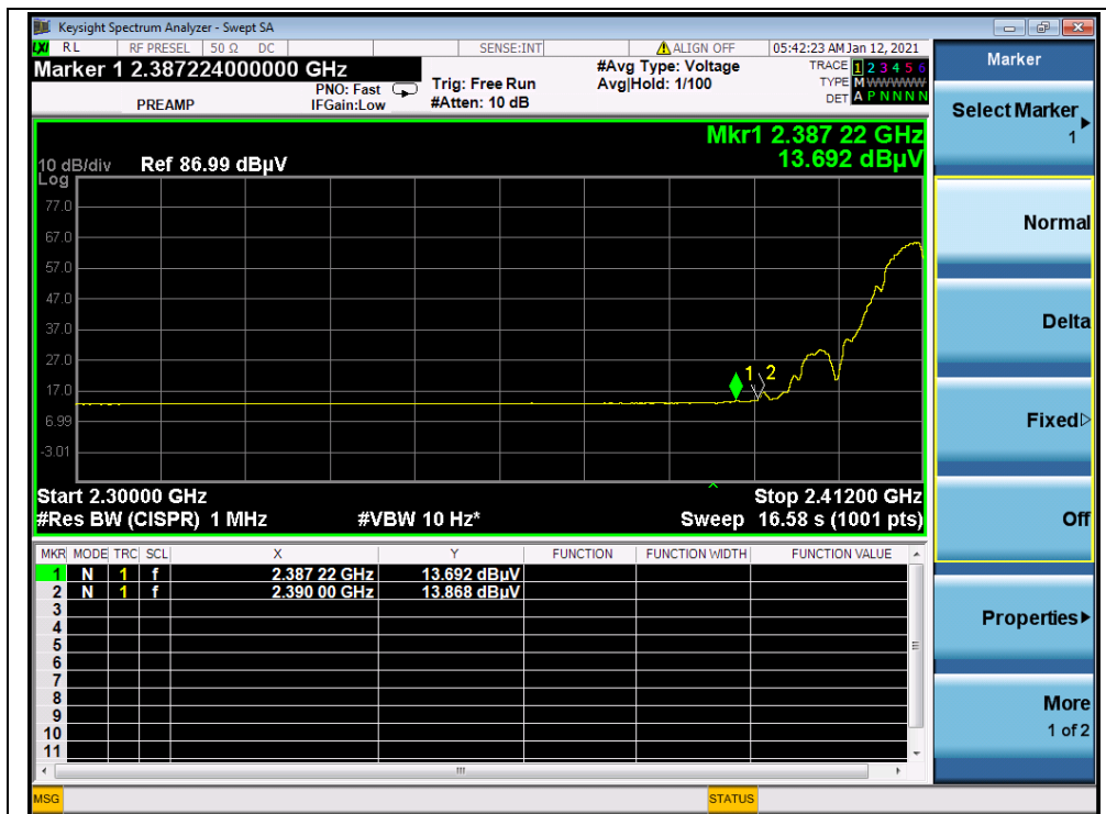
(AVG,Channel = 1, 802.11b)
