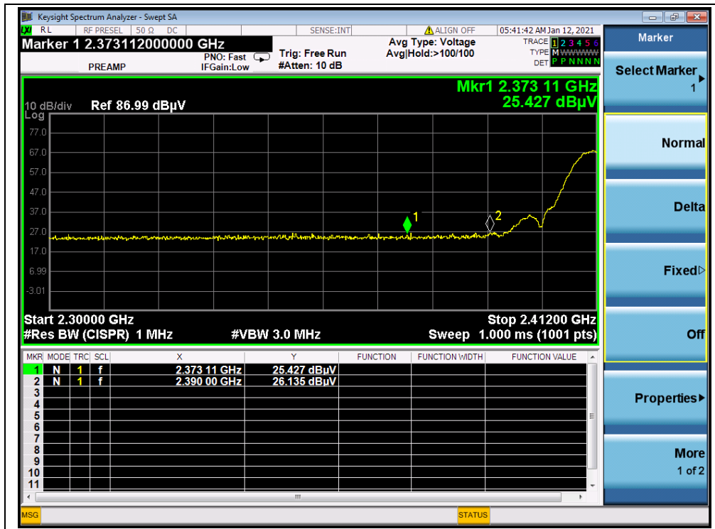
(PEAK,Channel = 1, 802.11b)
