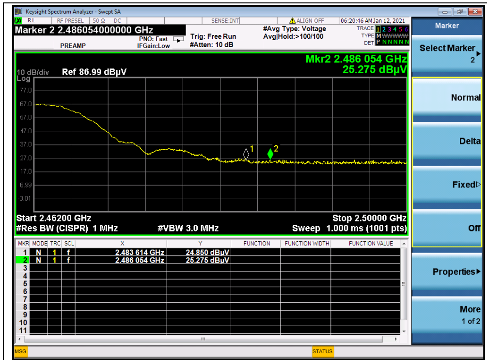
(PEAK,Channel = 11, 802.11b)
