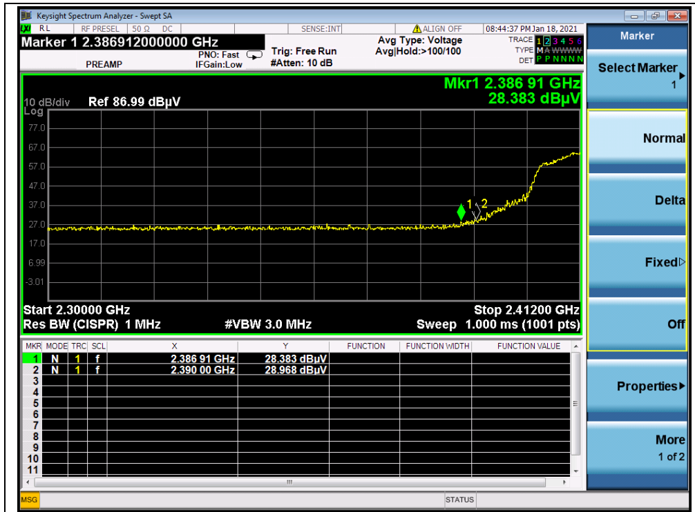
(PEAK,Channel = 1, 802.11n(HT20))
