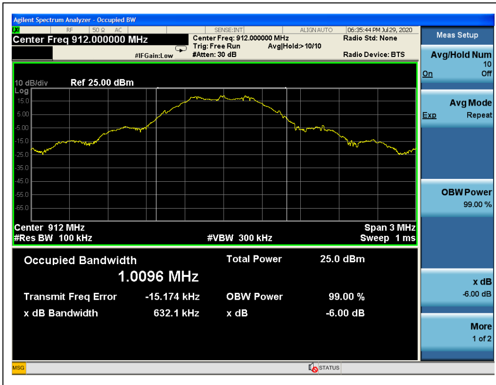
(912MHz)
