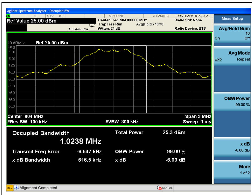
(904MHz)
