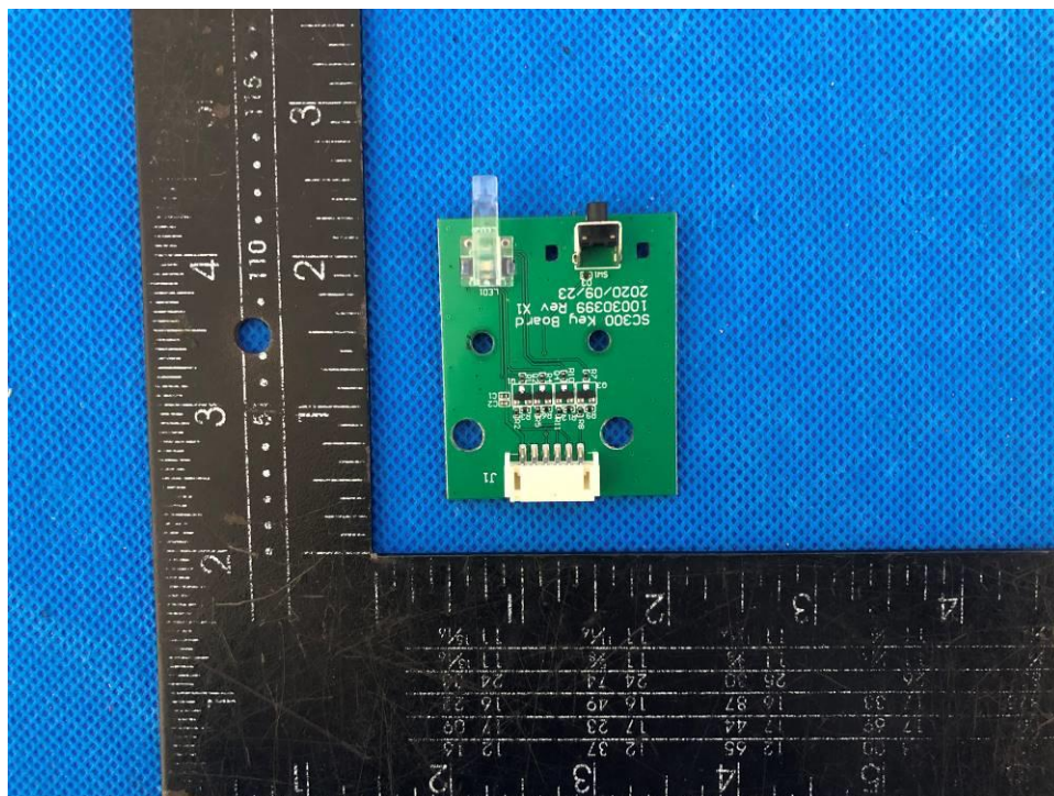
Figure 10. Top view of button board
