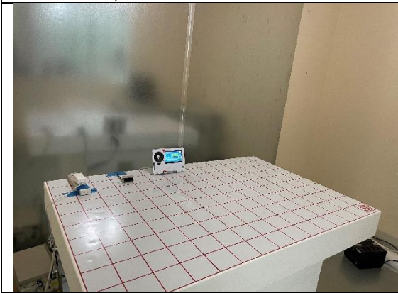
Conducted Emission-Front
