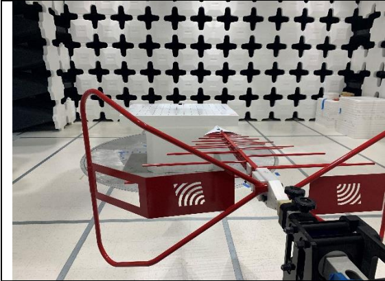
Radiated Spurious Emission-Below 1GHz- Front
