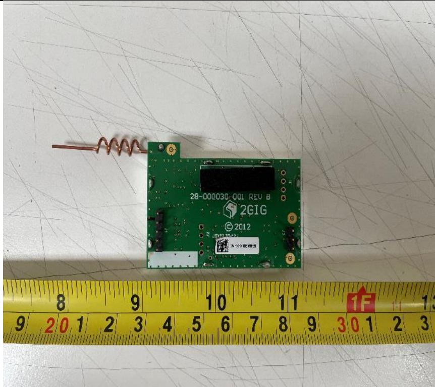
EUT Bottom View
