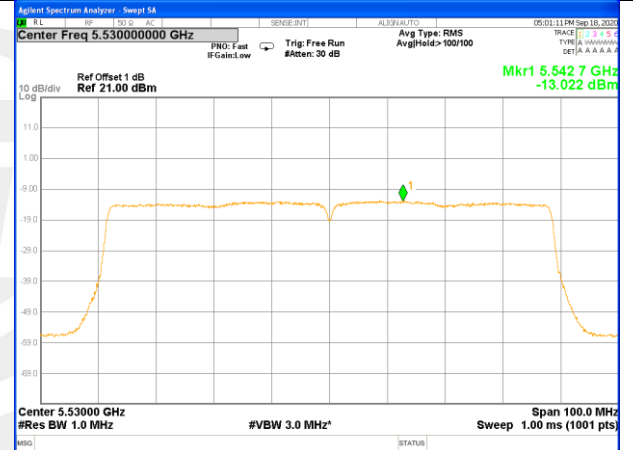
W56_11ac80_Lower_Power Spectrum Density
