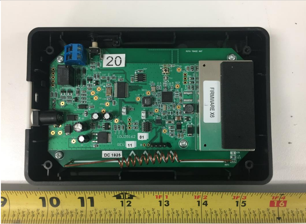
EUT Cover Off View-Top
