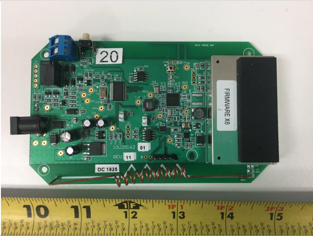
Main PCBA – Top View
