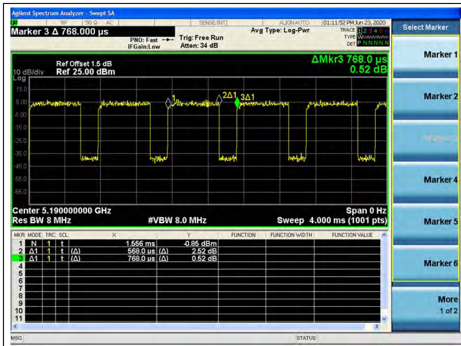
(CH38_5190MHz_802.11n(HT40))
