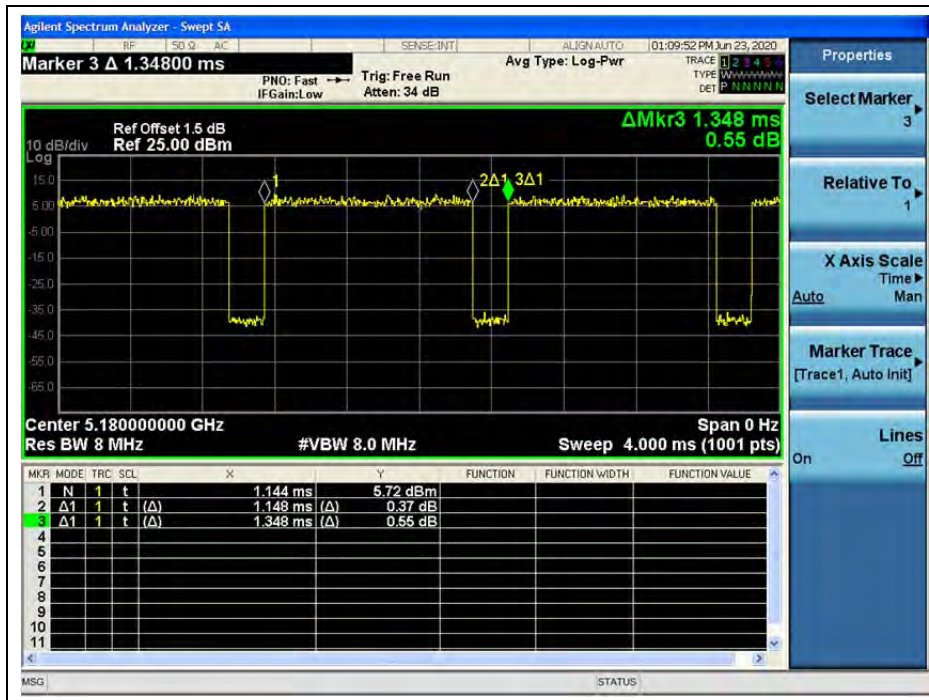
(CH36_5180MHz_802.11n(HT20))
