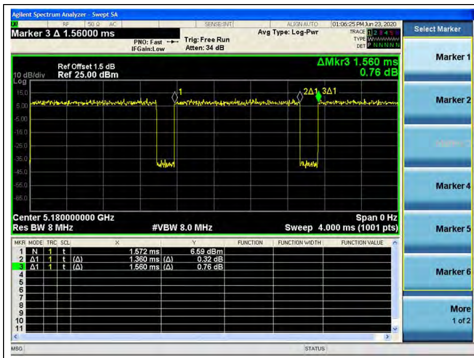
(CH36_5180MHz_802.11a)
