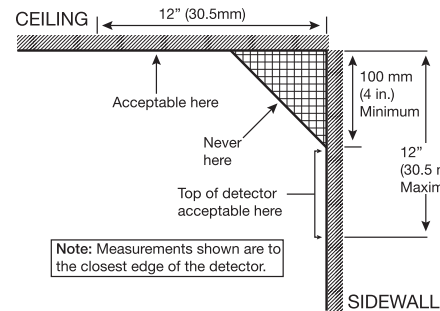
Fig 6. Example of proper mounting for Detectors
