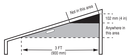
Fig 7. Example of proper mounting for Detectors with sloped ceilings
