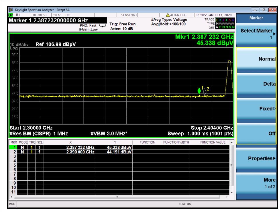
(AVG, Channel = 0)
