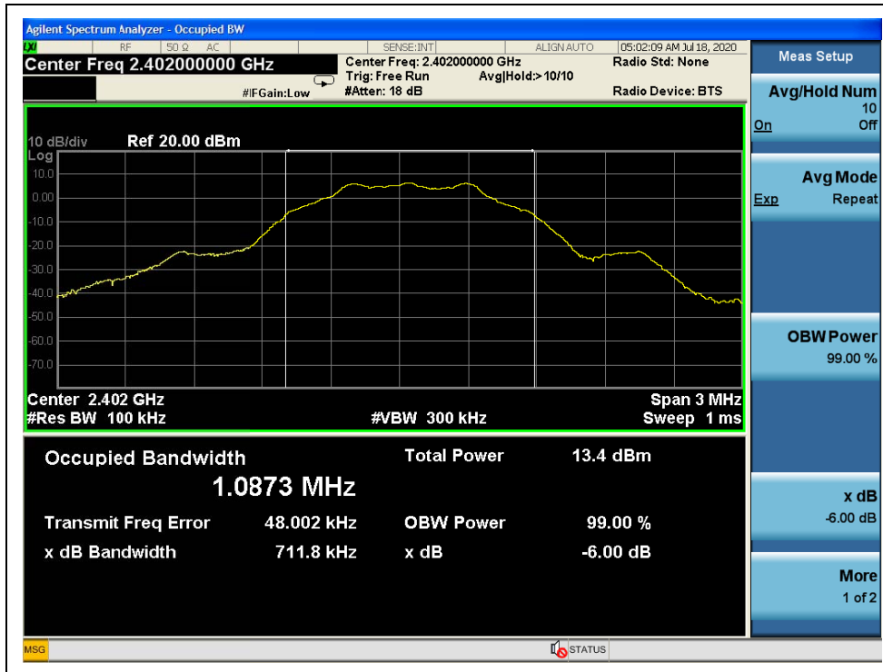
(Channel 0, 2402MHz)
