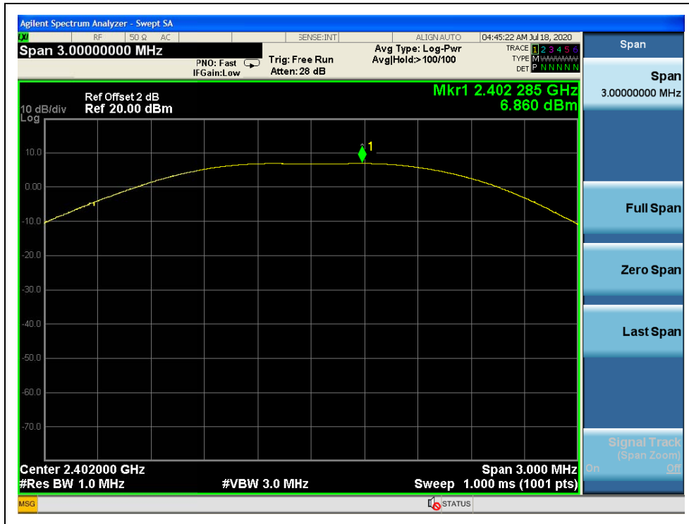
(Channel 0, 2402MHz)
