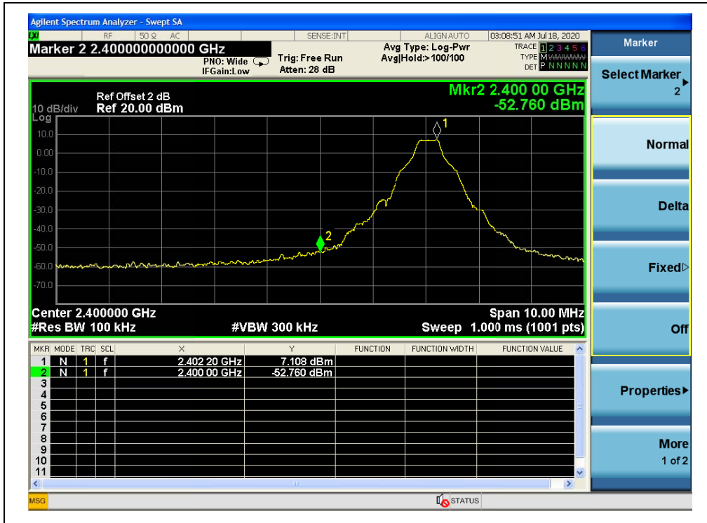
(Channel = 0, Band edge,GFSK Mode)
