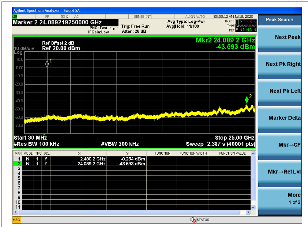
(Channel = 78, 30MHz to 25GHz, 8-DPSK)
