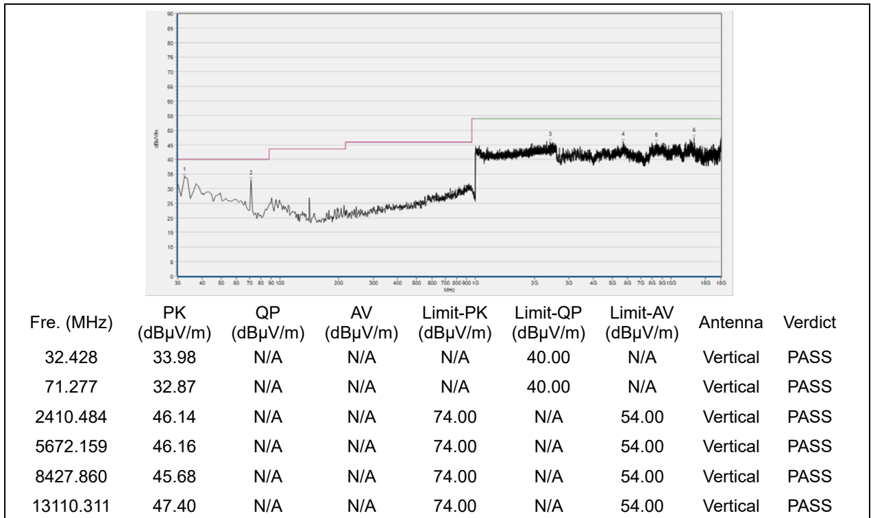
(30MHz to 18GHz, Antenna Vertical,8-DPSK, channel 0)
