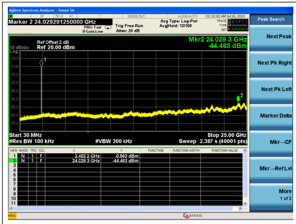
(Channel = 0, 30MHz to 25GH, 8-DPSK)
