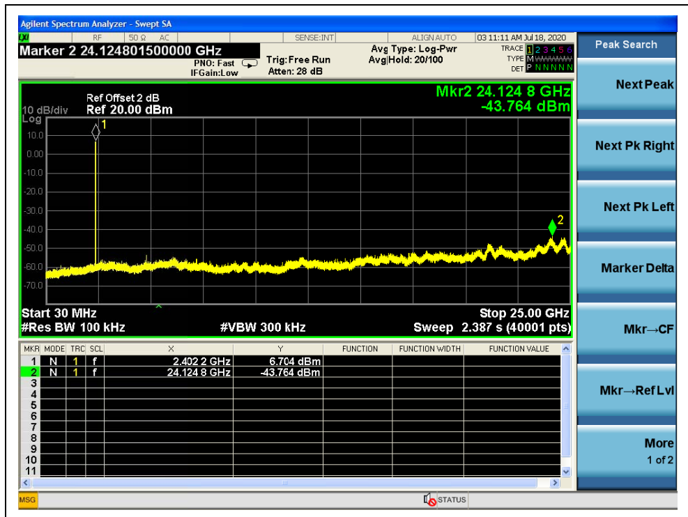
(Channel = 0, 30MHz to 25GHz, GFSK Mode)
