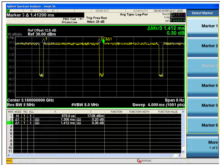
(CH36_5180MHz_802.11n(HT20))
