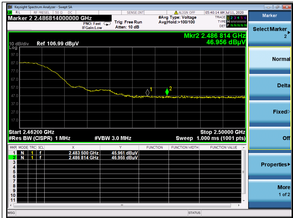
(PEAK,Channel = 11, 802.11b)
