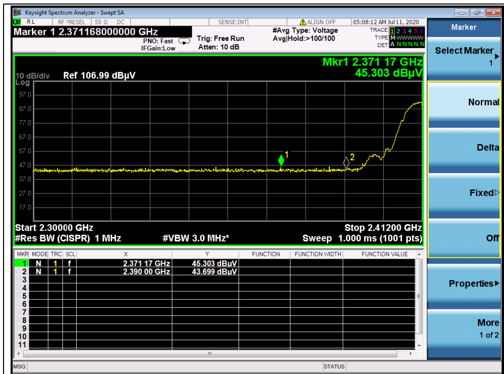
(AVG,Channel = 1, 802.11b)
