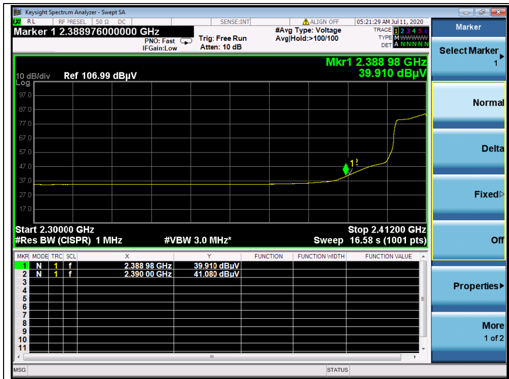
(AVG,Channel = 1, 802.11n(HT20))
