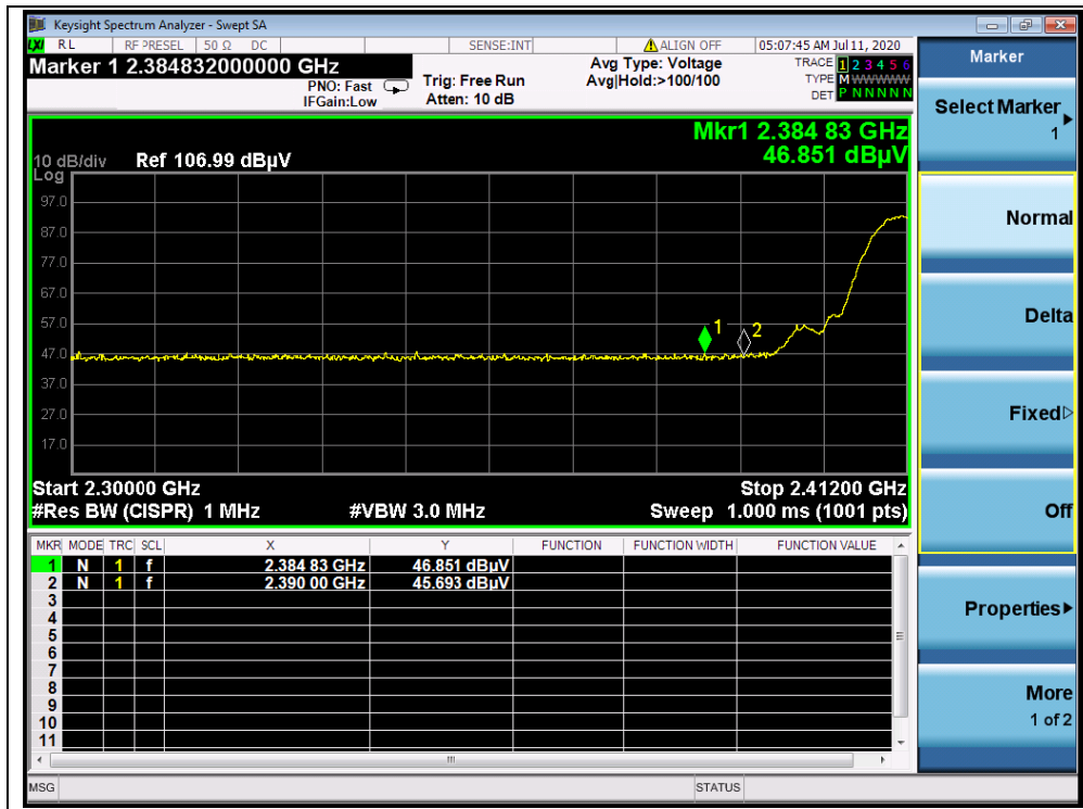
(PEAK,Channel = 1, 802.11b)
