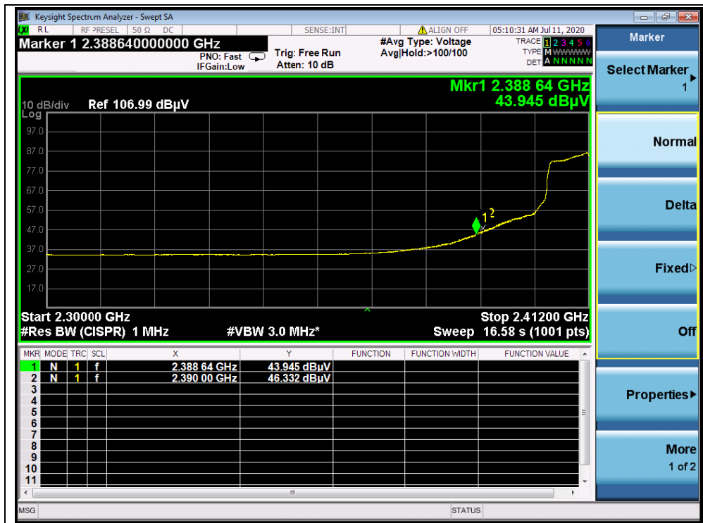
(AVG,Channel = 1, 802.11g)
