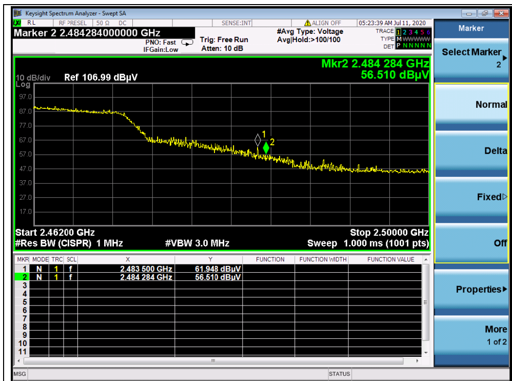
(PEAK,Channel = 11, 802.11n(HT20))
