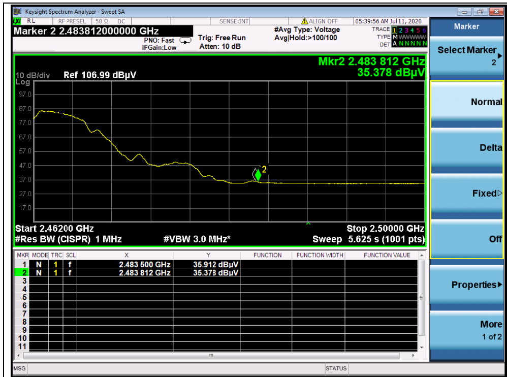
(AVG,Channel = 11, 802.11b)
