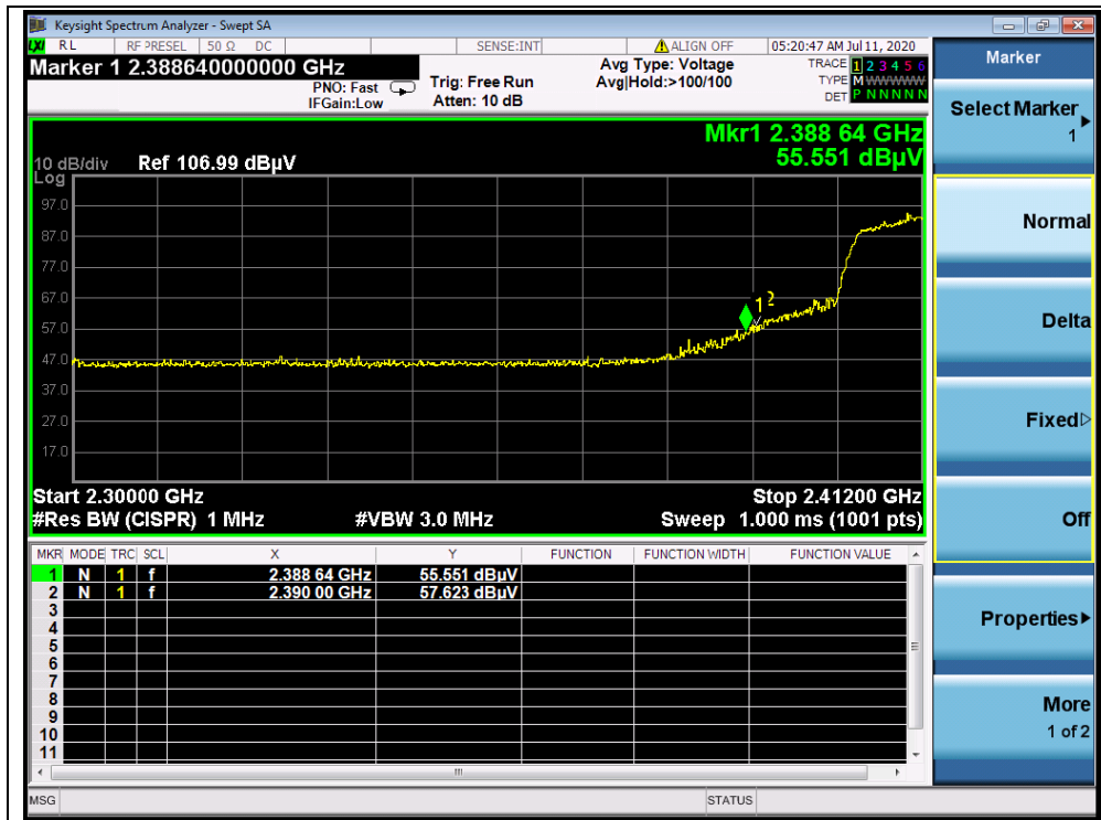
(PEAK,Channel = 1, 802.11n(HT20))
