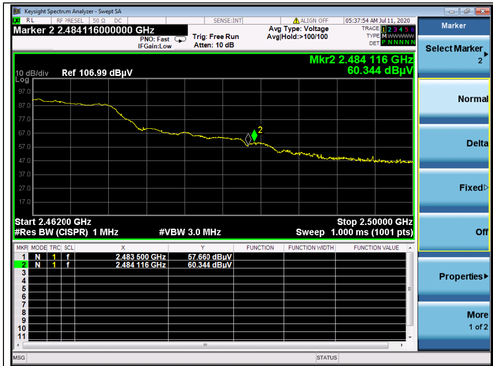
(PEAK,Channel = 11, 802.11g)
