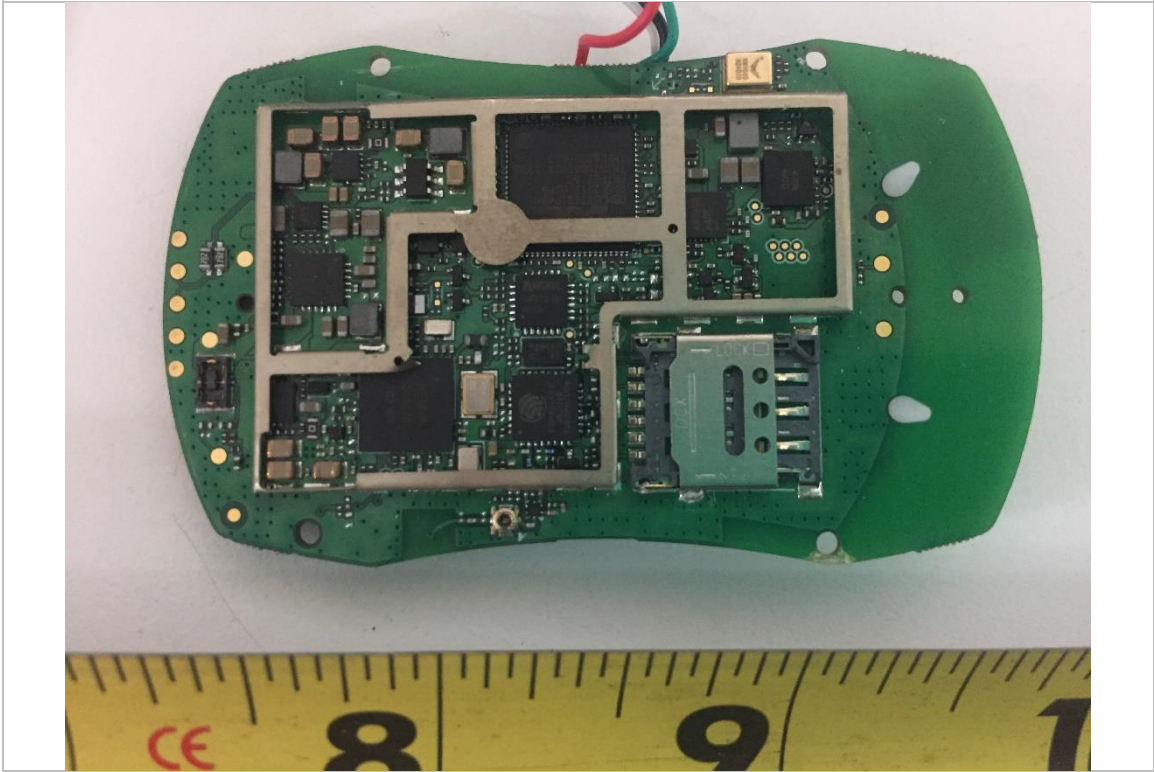
EUT Cover Off View without shielding – Bottom
