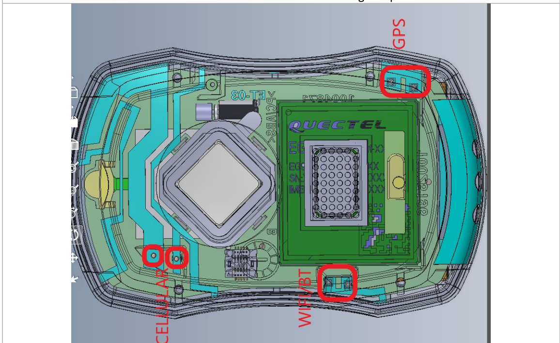
Libris Antenna Connections
