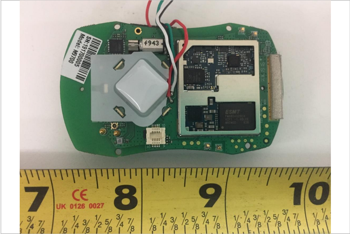
EUT Cover Off View without shielding – Top
