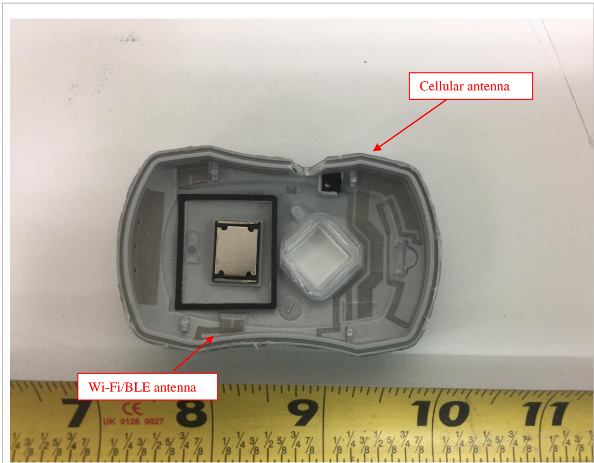
EUT Cover Off View without shielding – Top
