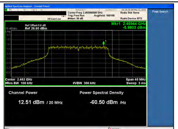
11n-20MHz-PSD-High-MCS7
