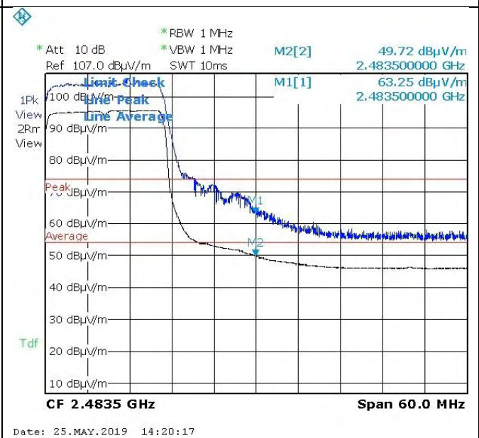
802.11g 2462M-High
