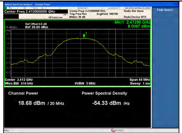
11b-PWR-Low-11Mbps
