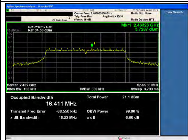
11g-6dB BW-High-6Mbps
