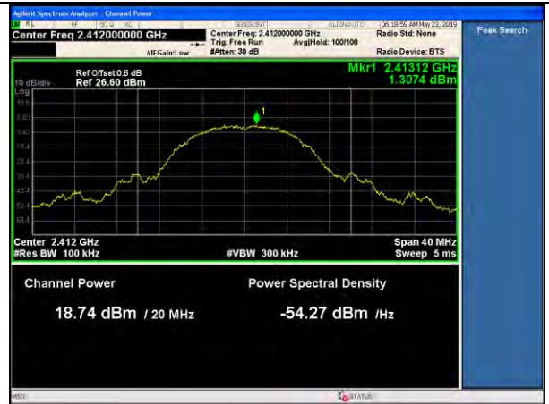
11b-PSD-Low-11Mbps
