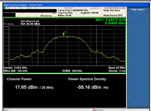
11b-PSD-High-11Mbps
