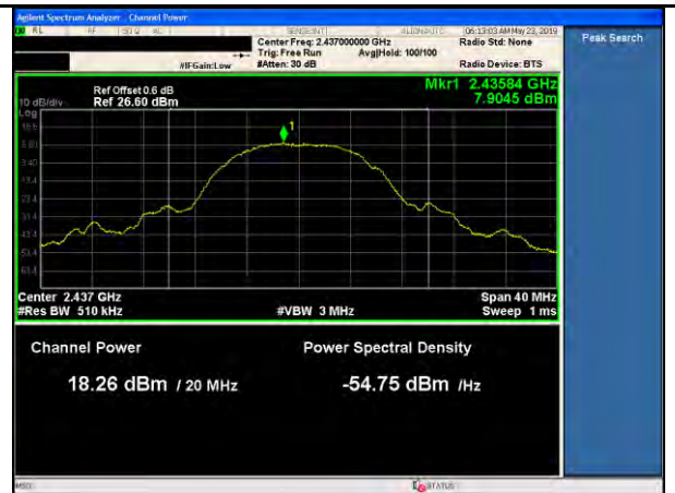
11b-PWR-Mid-11Mbps
