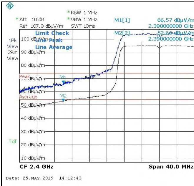
802.11n 2412M-Low
