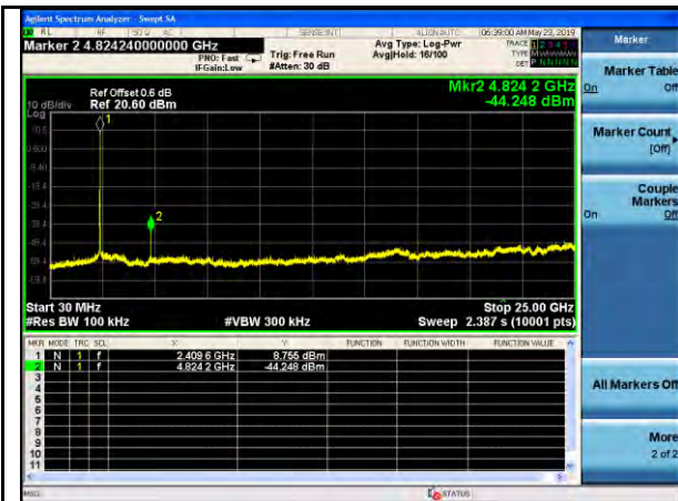
11b-Out Of Band Emission-Low
