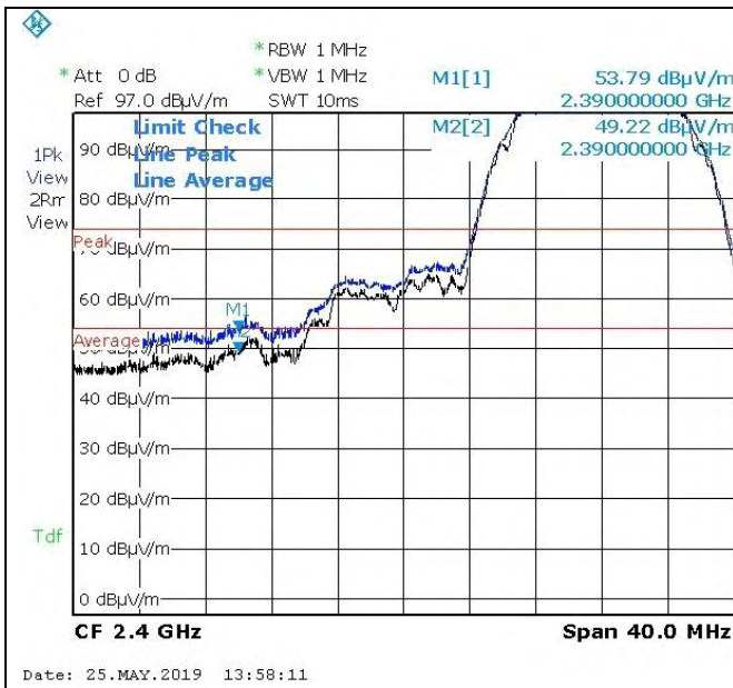
802.11b 2412M-Low
