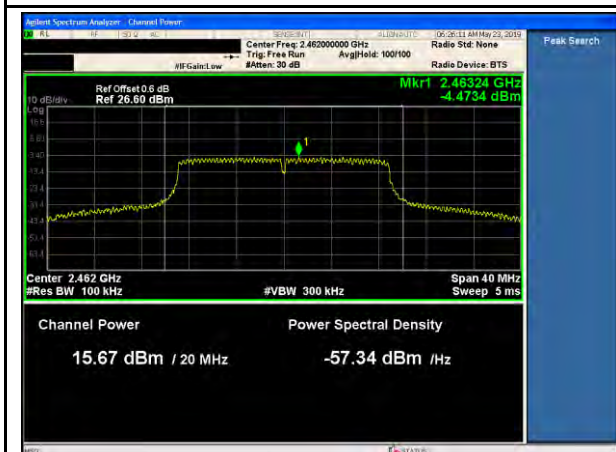
11n-20MHz-PSD-High-MCS0
