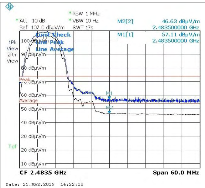
802.11b 2462M-High
