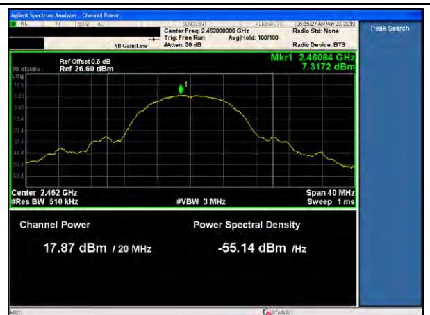
11b-PWR-High-11Mbps
