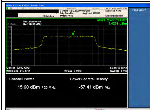
11n-20MHz-PWR-High-MCS0
