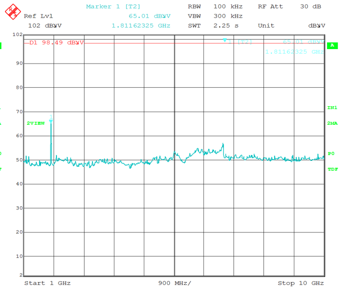
Comment A: Conducted Spurious Middle Channel
