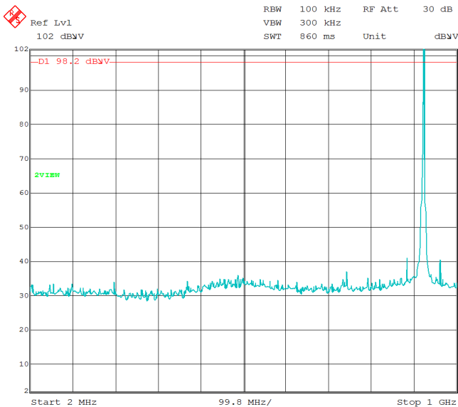
Comment A: Conducted Spurious High Channel
