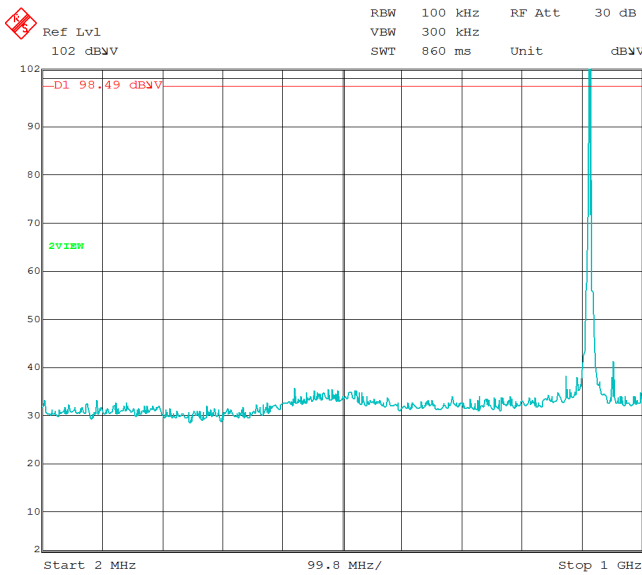
Comment A: Conducted Spurious Middle Channel
