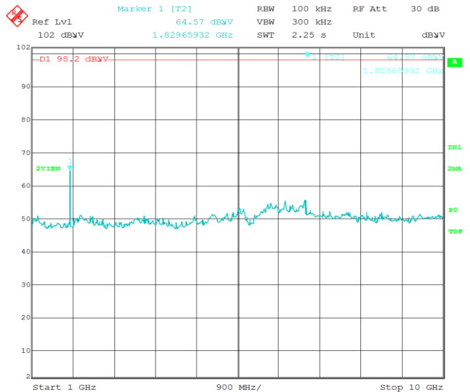
Comment A: Conducted Spurious High Channel
