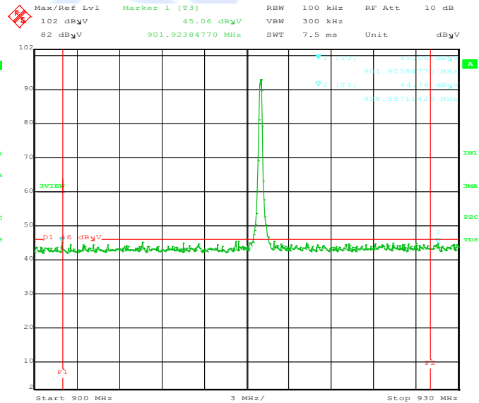
Comment A: Band Edge 916MHz Vertical Date: 17.MAY.2016 13:10:43
