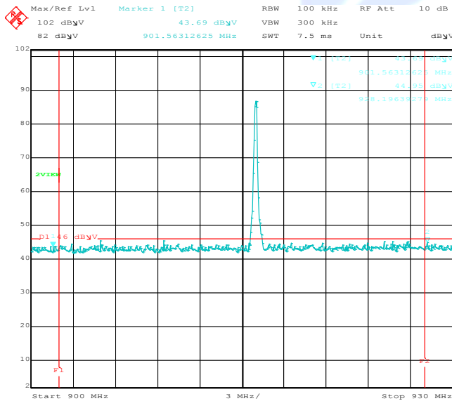
Comment A: Band Edge 916MHz Horizontal Date: 17.MAY.2016 13:03:06
