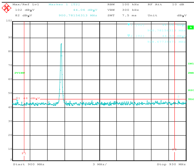
Comment A: Band Edge 908.42MHz Horizontal Date: 17.MAY.2016 13:39:22
