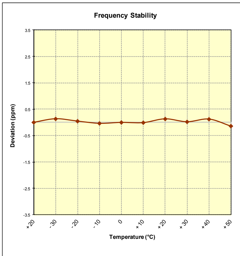
Figure 6-9. Frequency Stability Graph (PCS CDMA Mode – Ch. 600)
