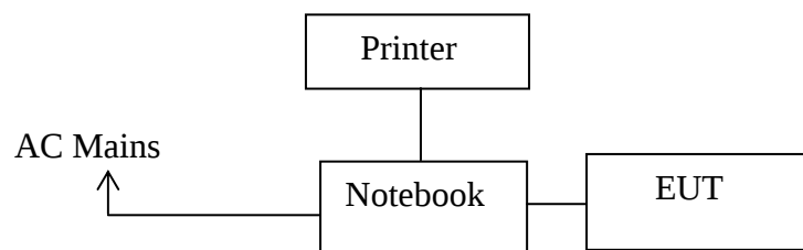
Figure 2 EUT Setup of Connect to PC mode
