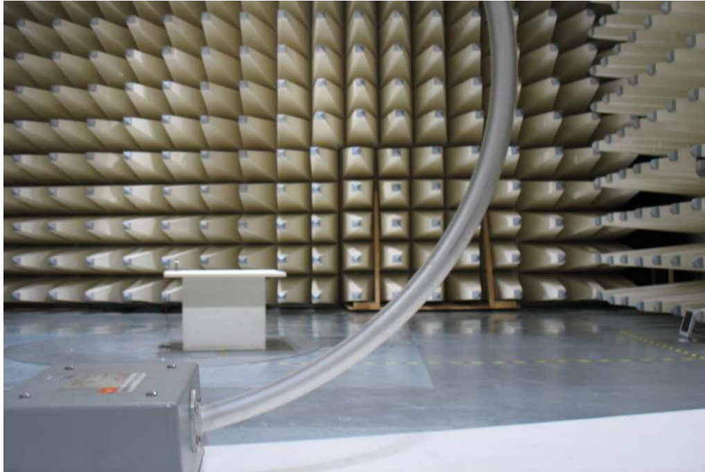
Photo 3: Radiated Emissions
