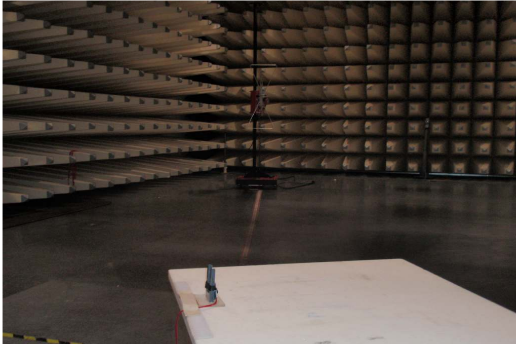
Photo 1: Radiated Emissions
