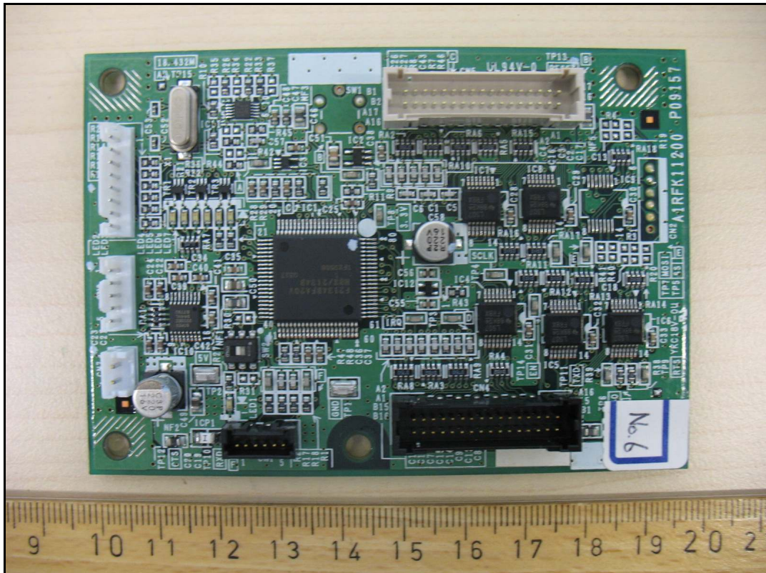
Photo 6: Control board
