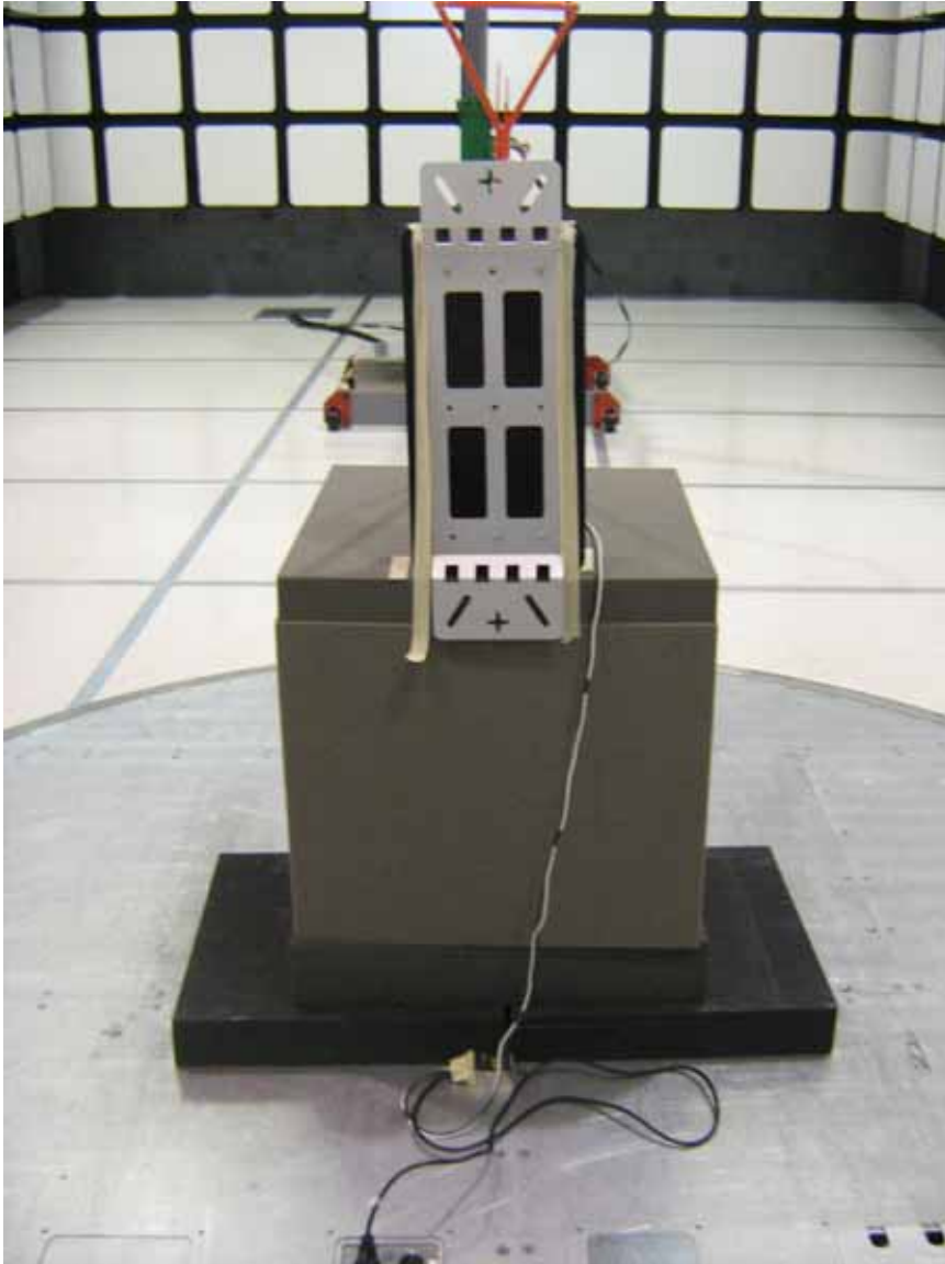
Figure 2: Test Setup for 30 MHz to 1000MHz (Rear View)
