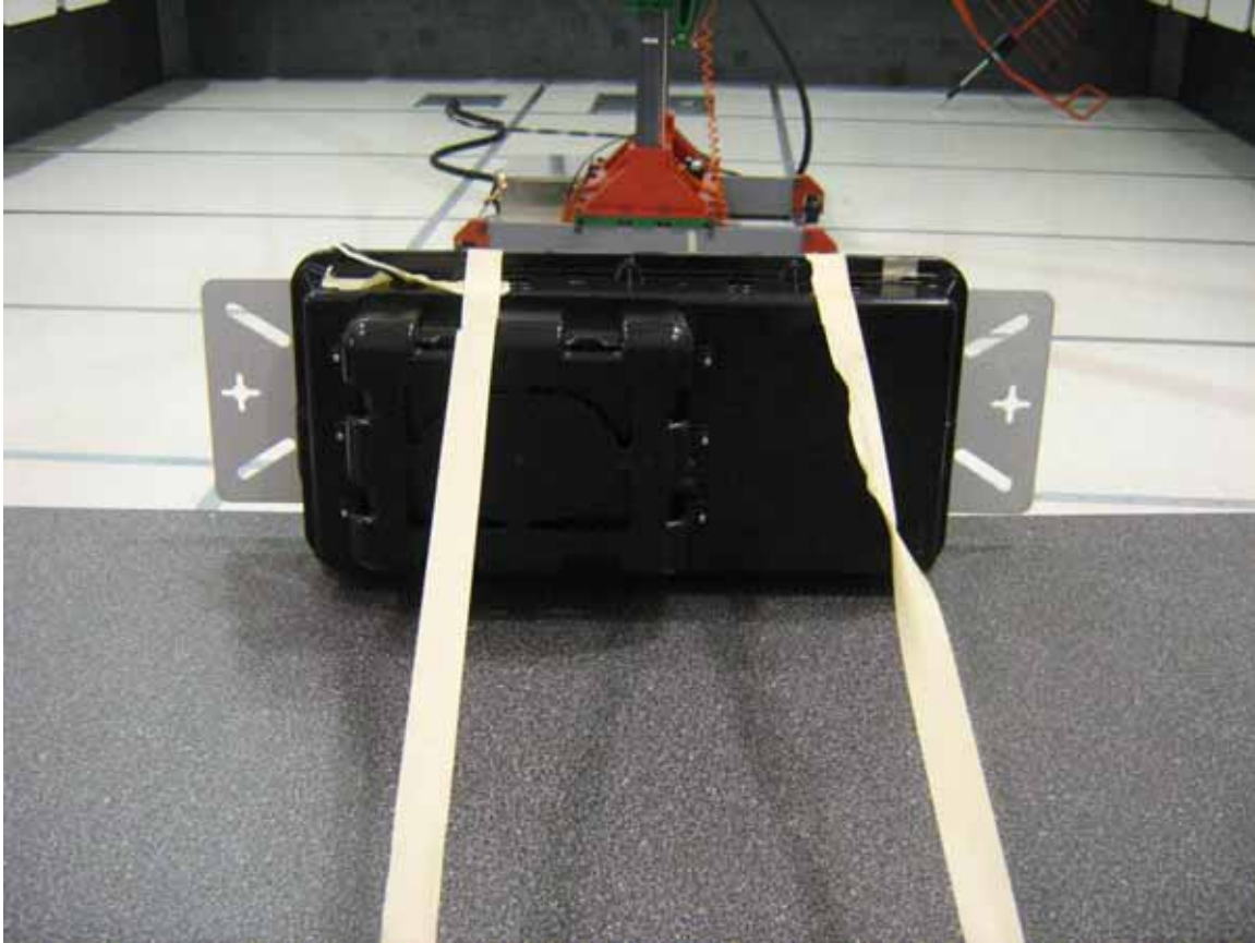
Figure 6: Radiated Emission Setup with EUT on Y-Axis
