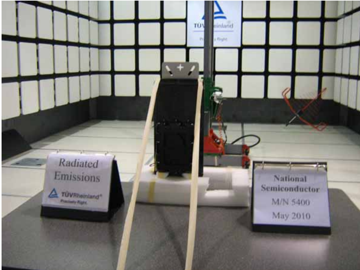
Figure 7: Radiated Emission Setup with EUT on Z-Axis
