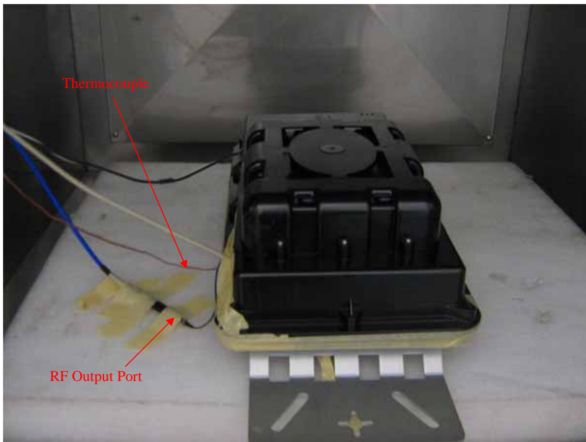
Figure 9: Photo of Test Setup for SM5400, Voltage and Temperature Variation.
