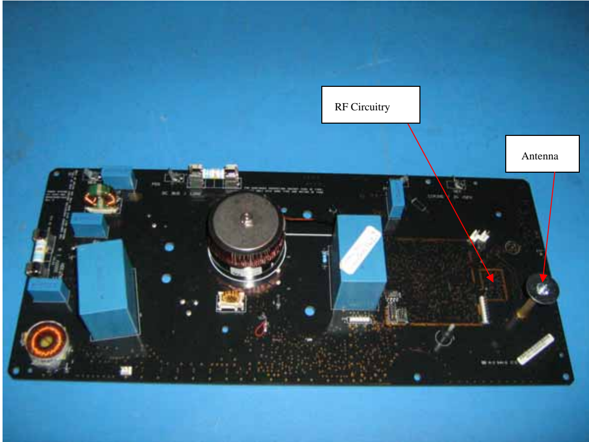
Figure 1: Internal Photo of SM5400 without Plastic Enclosure (Component Side)
