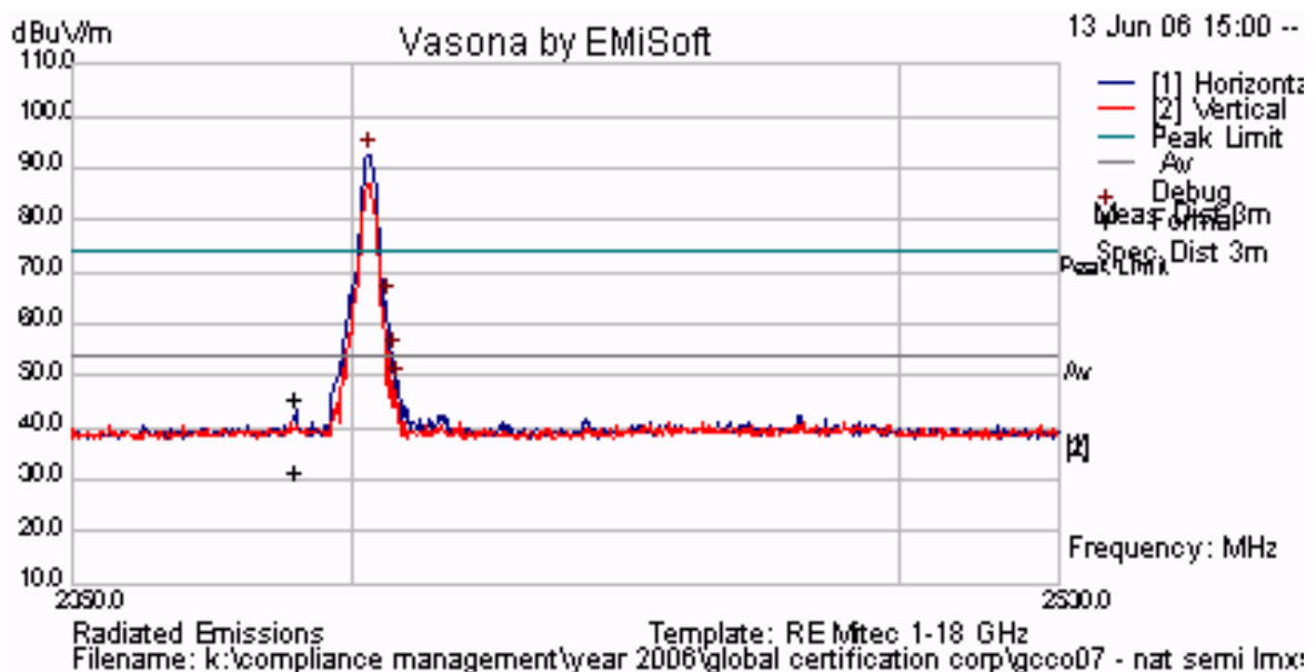
Plot 46 Channel 1 - Lower Band Edge, Peak Emission = 92.71 dBµV/m
