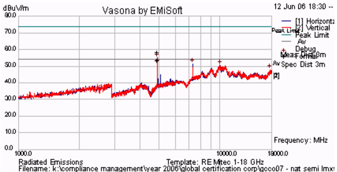
Plot 29 Radiated Emissions for Channel 2441 Antenna #2 - 2 dBi External Wamel Monopole
