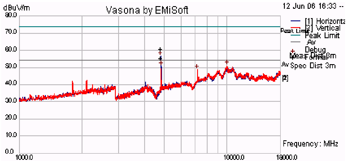
Plot 28 Radiated Emissions for Channel 2402 Antenna #2 - 2 dBi External Wamel Monopole
