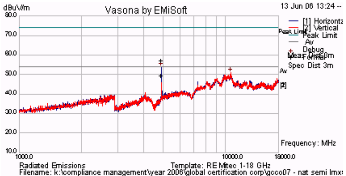
Plot 32 Radiated Emissions for Channel 2441 Antenna #3 - 0.5 dBi Integral Antenna Factor
