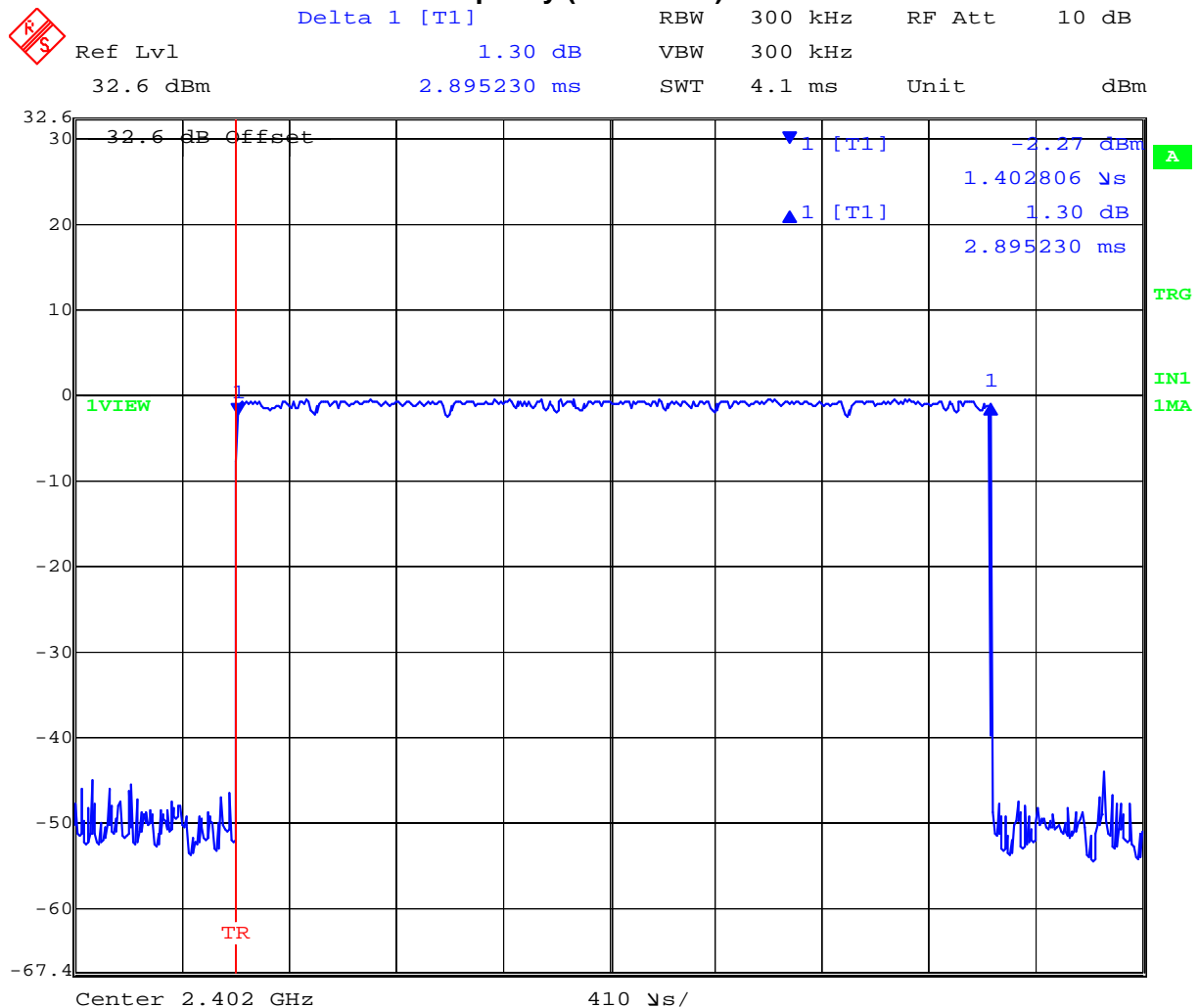
Plot 11 Channel Occupancy (dwell time) Ch 1 2402 MHz
