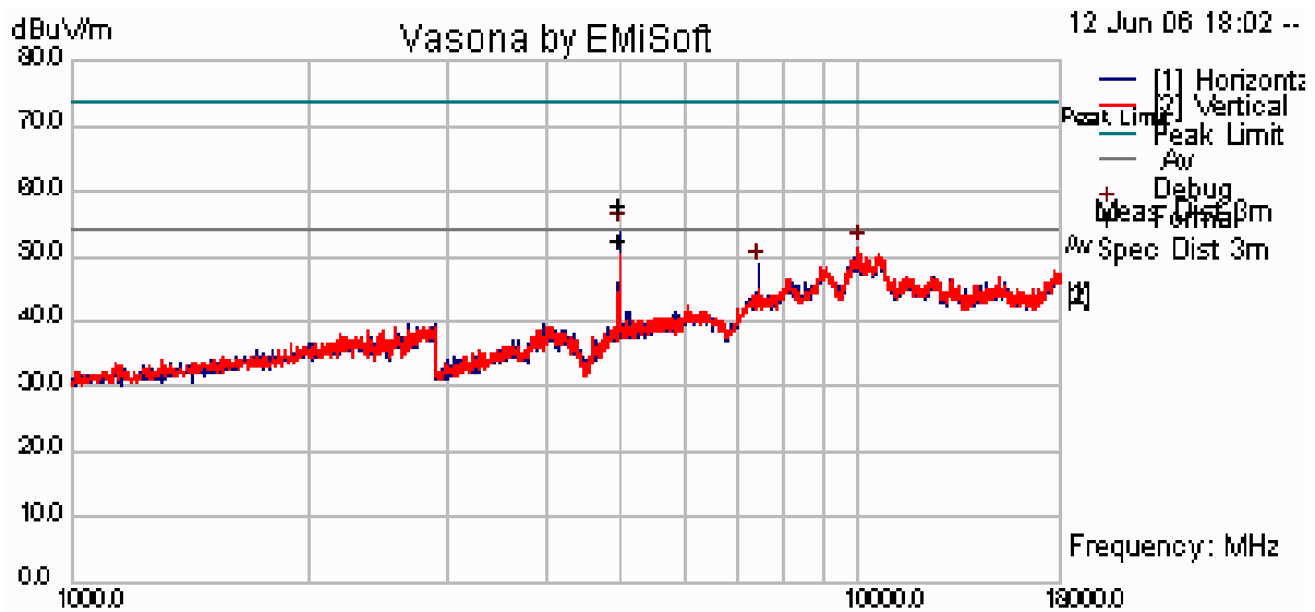
Plot 30 Radiated Emissions for Channel 2480 Antenna #2 - 2 dBi External Wamel Monopole
