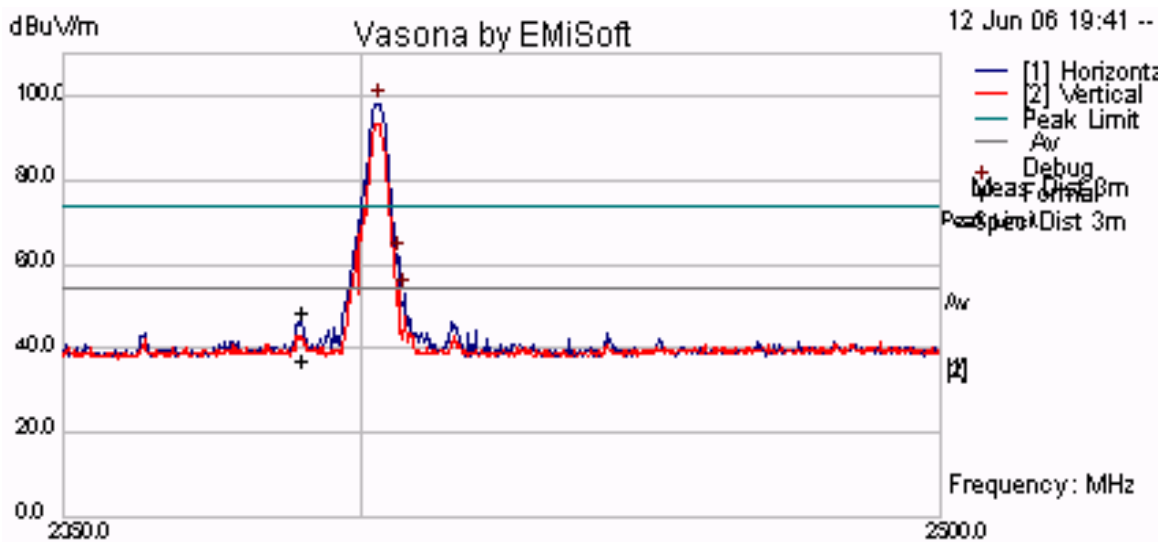
Plot 37 Channel 1 - Lower Band Edge, Peak Emission = 98.2 dBuV/m
