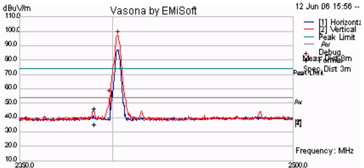
Plot 40 Channel 1 - Lower Band Edge, Peak Emission = 97.04 dBuV/m
