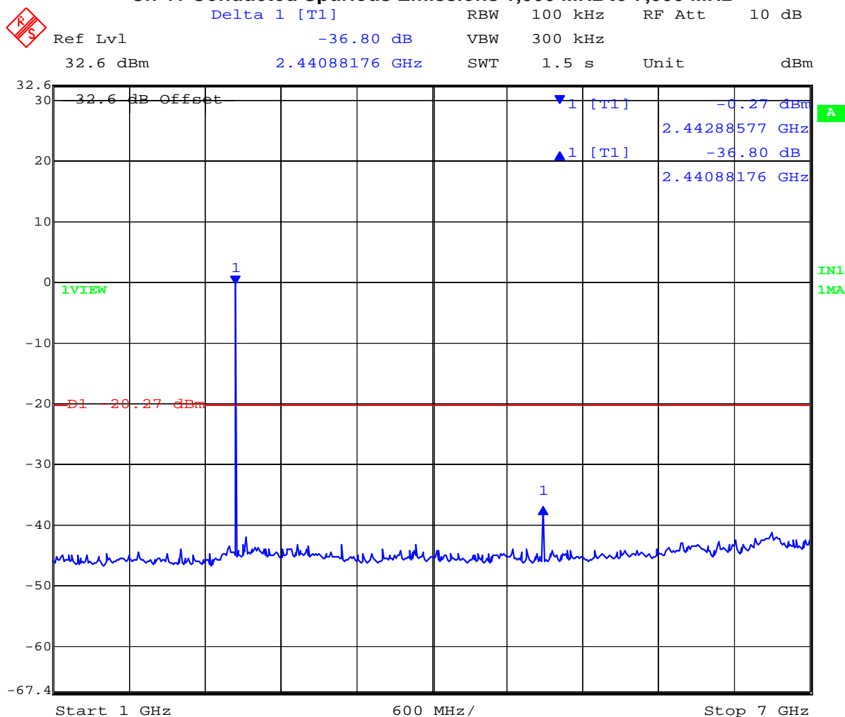
Plot 21 Ch 41 Conducted Spurious Emissions 1,000 MHz to 7,000 MHz
