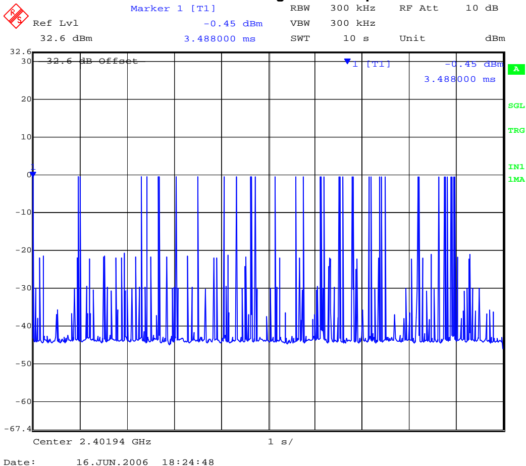
Plot 08 Channel Occupancy Ch 1 2402 MHz 30 times visited during 10 second period
