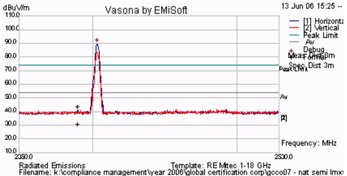
Plot 43 Channel 1 - Lower Band Edge, Peak Emission = 89.54 dBuV/m
