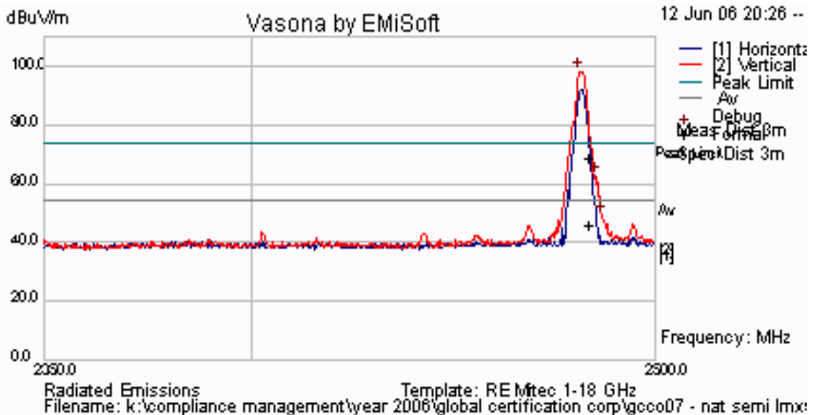
Plot 41 Channel 80 – Upper Band Edge, Peak Emission = 98.34 dB \mu V/m
