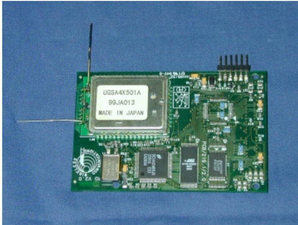
Photo 2 - RF PCB Component Side
