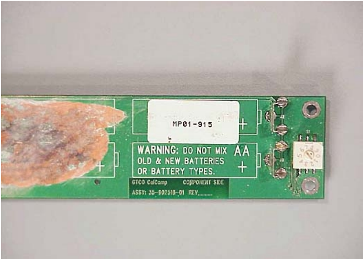
Close-up of top of board section 4
