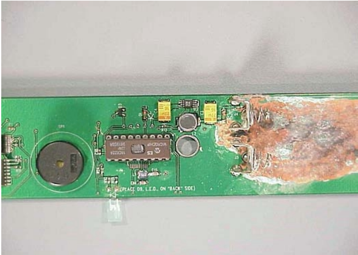
Close-up of top of board section 3
