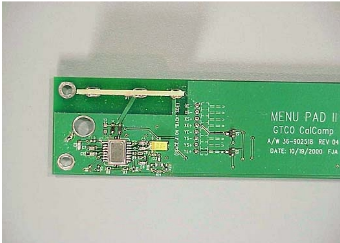
Close-up of top of board section 1
