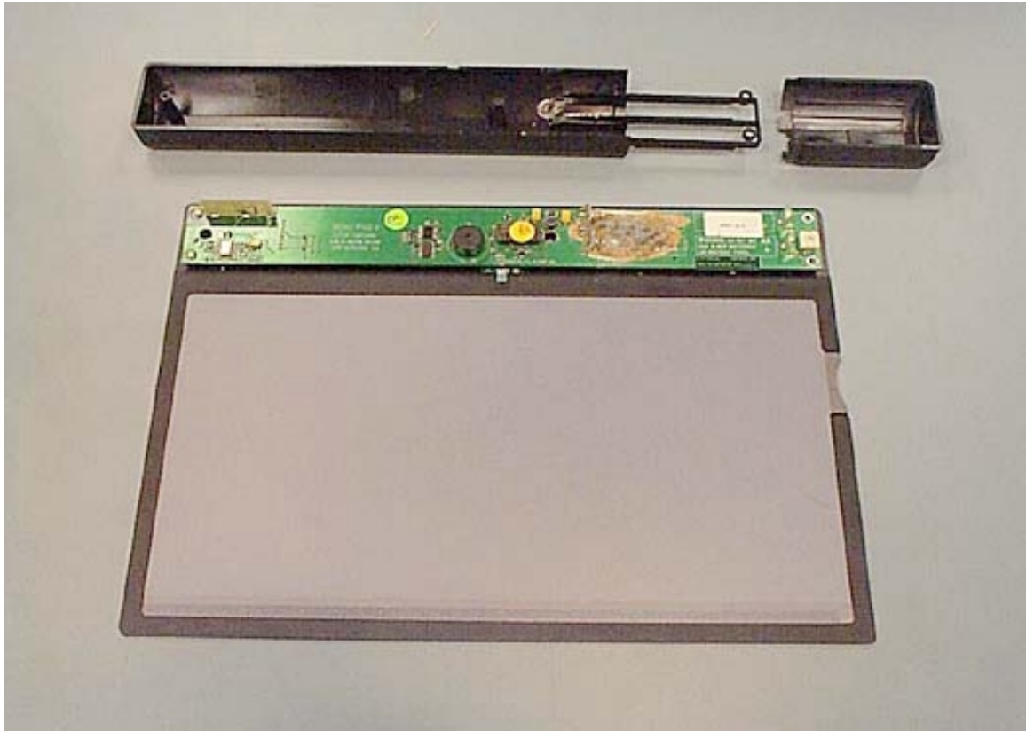
Cover off showing top of board
